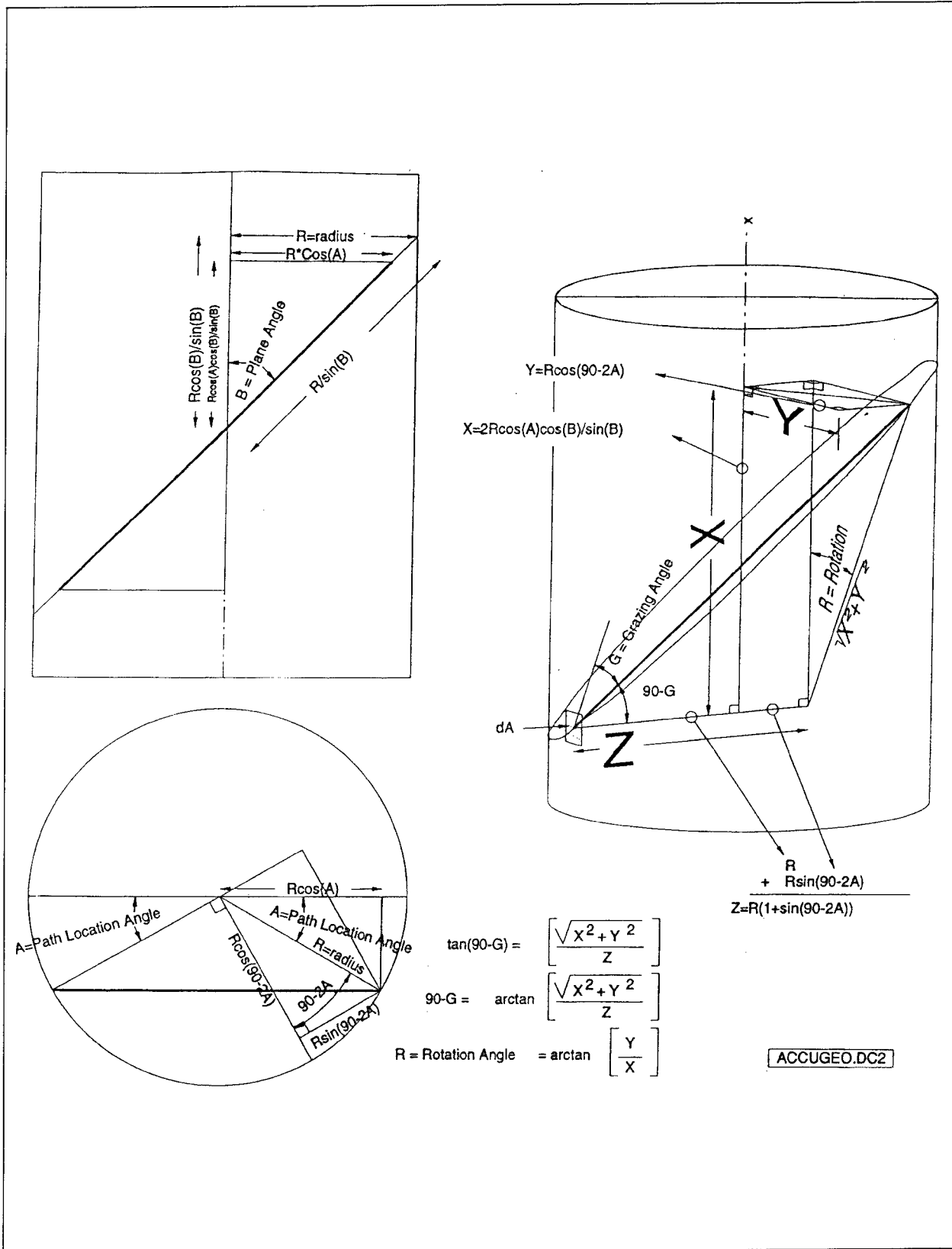
Figure A3. Grazing angle geometry for chordal path
