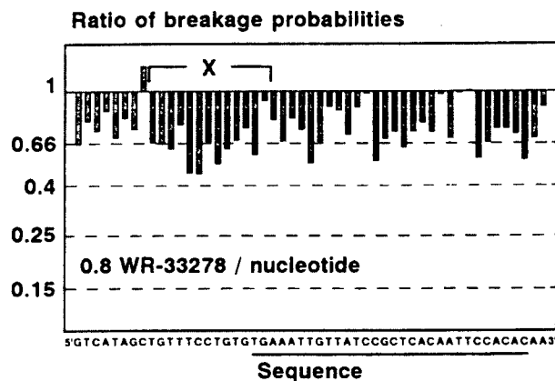
Figure 6. Ratios of the probability of strand breakage at each nucleotide along a part of the 80 bp DNA fragment irradiated in the presence and in the absence of WR-33278. Irradiation dose, 80 Gy fast neutrons. Anoxic conditions. The results are those of a typical experiment out of five rendering similar patterns. The experimental error in the determination of the areas of peaks in the densitogram of gels is <3\% . Underlined, the sequence of the modeled 30 bp fragment.
