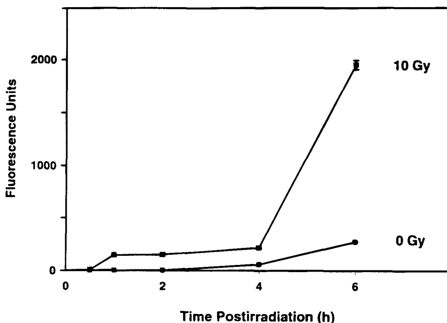
FIGURE 6 Effect of 10 Gy ^{60}\text{Co} gamma radiation on Trolox-induced DCFH-DA oxidation.
