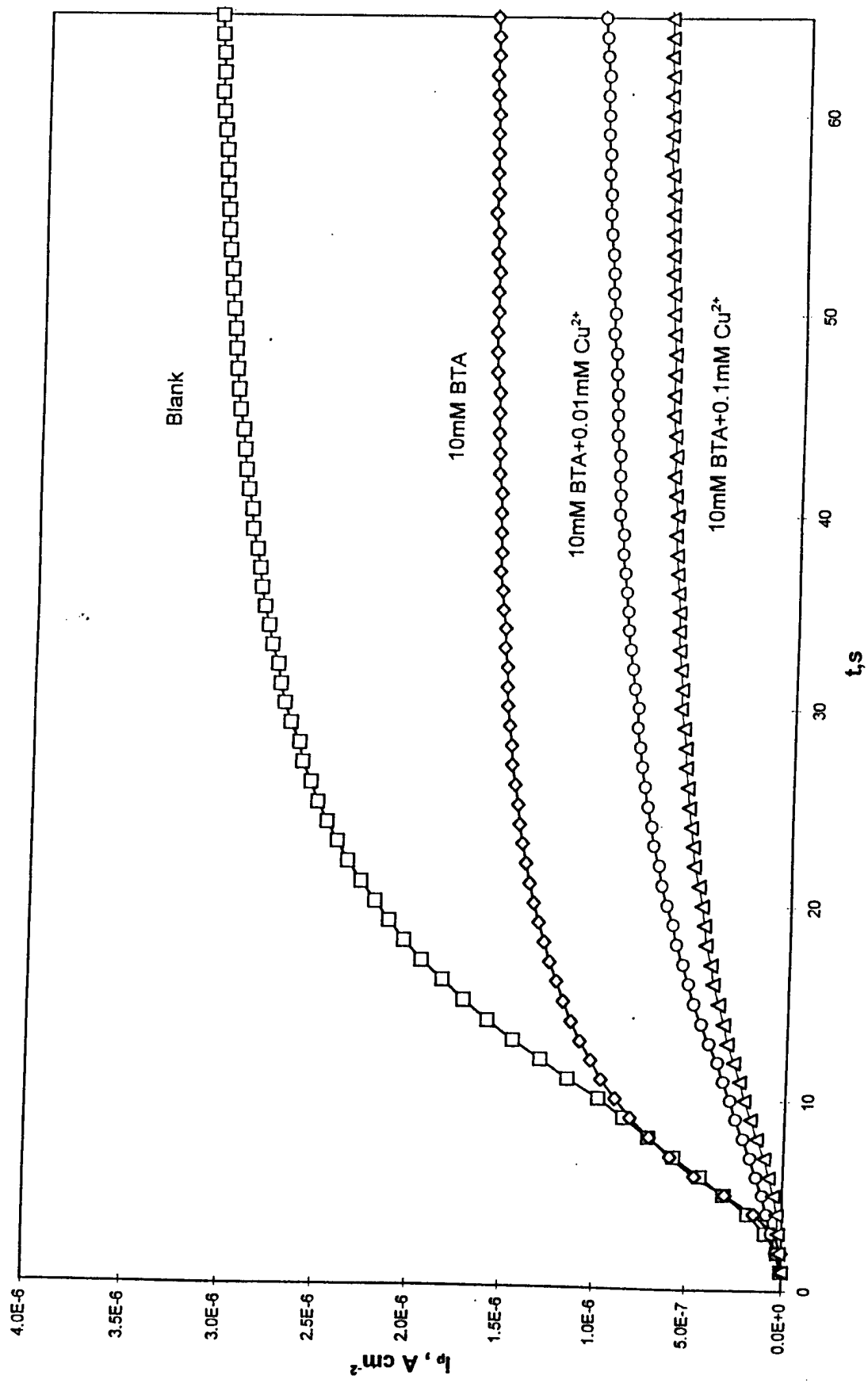
Figure 10 Hydrogen permeation transients obtained at a charging current density of 1.25 mA cm -2 for different charging solution compositions.
