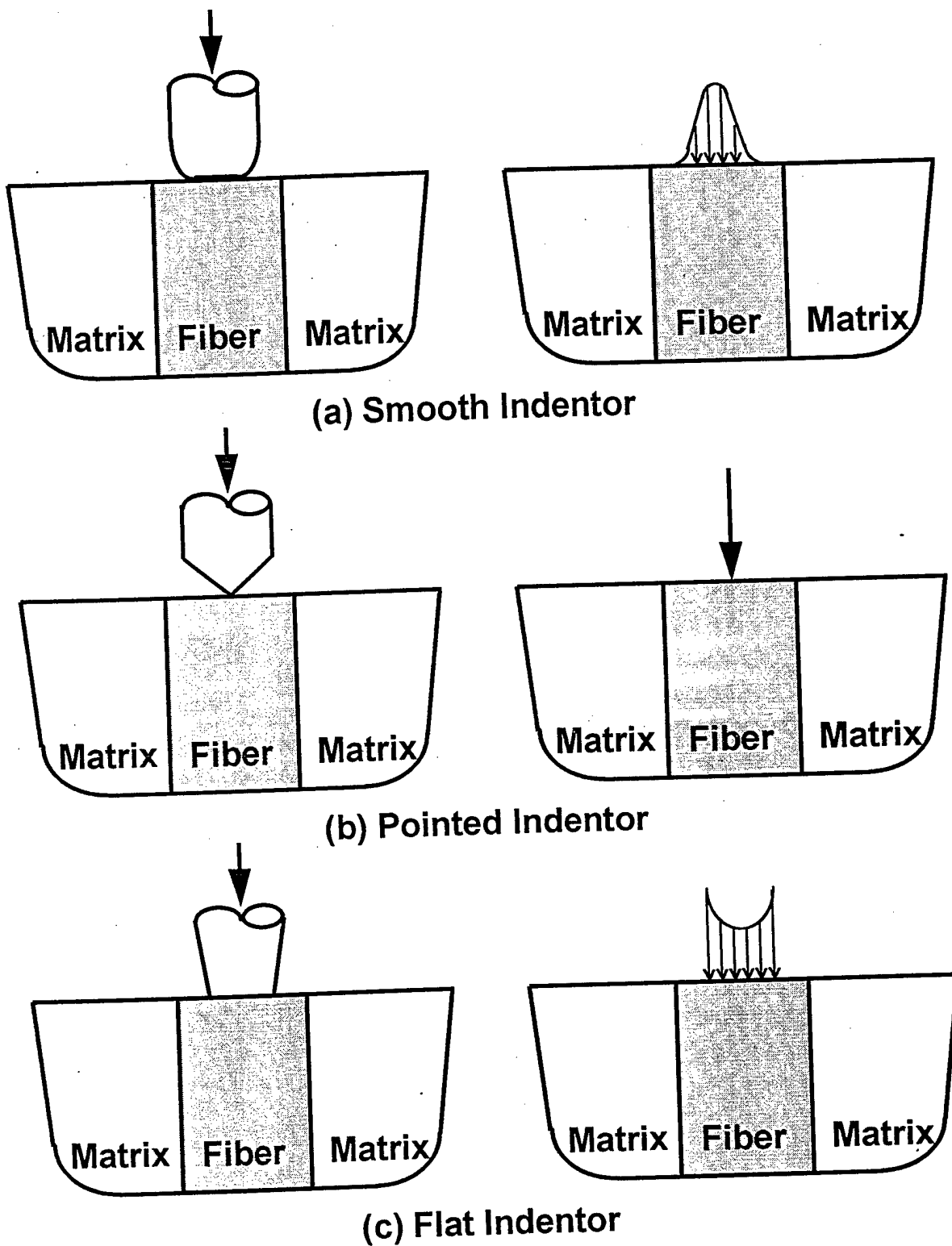
Figure 2. Various indenter geometries and the approximated pressure distribution on the fiber.
