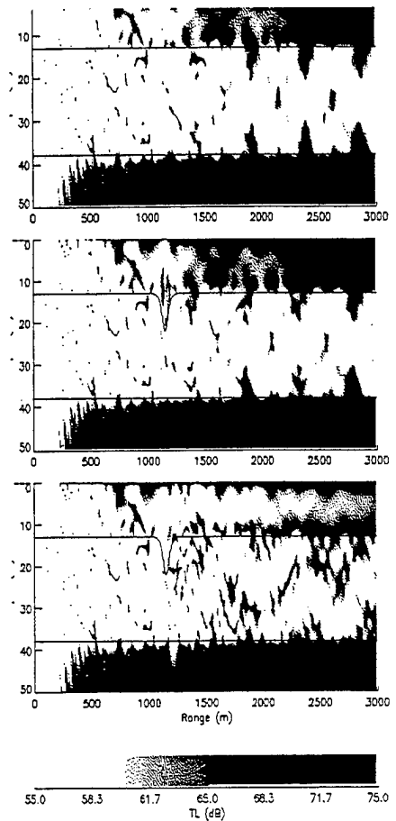
FIG. 3. Comparison of TL for 1-soliton environment at 940 Hz: range independent (topmost figure), adiabatic modes (middle), and coupled modes (bottom).
