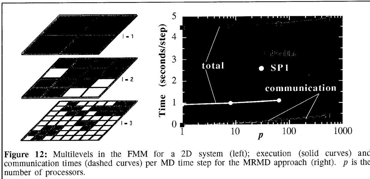
Figure 12 shows the performance of the MRMD approach on the 512-node Touchstone Delta machine at Caltech and the 128-processor IBM SP system at Argonne National Laboratory. The execution time scales linearly with the system size and the computation time dominates the communication time. Using MPI (Message Passing Interface), the MRMD has been ported to other parallel platforms as well.
