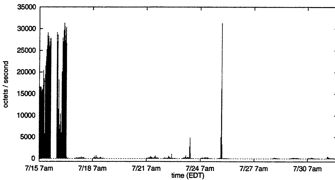
Figure 6. Traffic during the testing period from RL BTS to the COMPASS lab.
