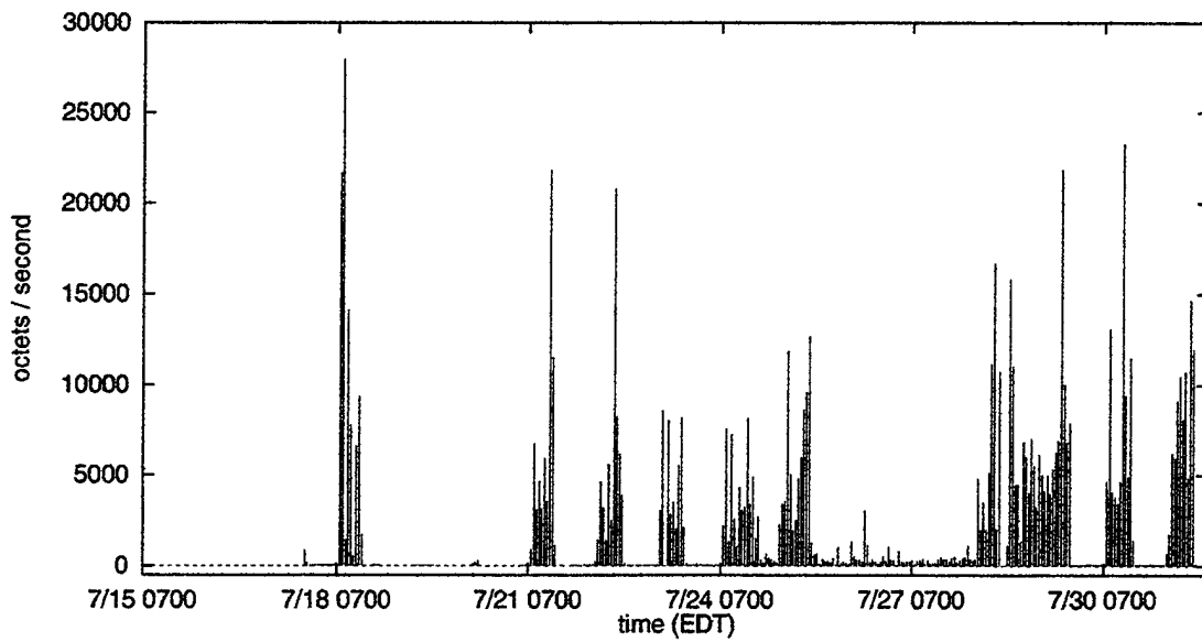
Figure 12. Multicast server traffic from NH95 to the COMPASS lab. Data collection started on 17 July at 1915 EDT.
