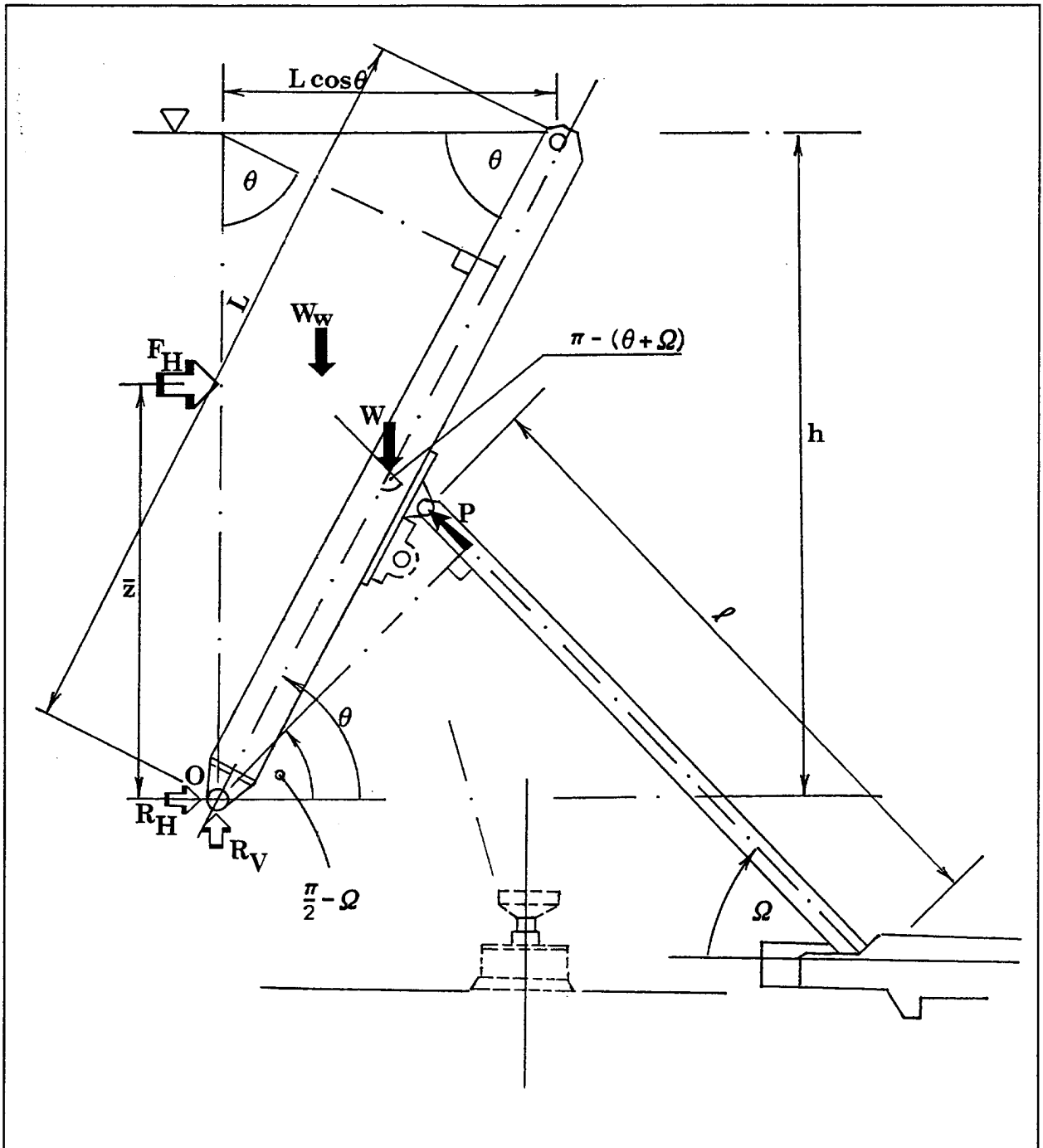
Figure 12. Equilibrium of forces on gate
