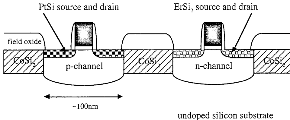
Fig. 3 Sketch of future \sim 25\text{nm} gate-length Schottky barrier CMOS inverter with buried, epitaxial, and self-planarized \text{CoSi}_2 local interconnects.
