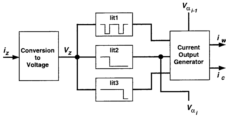
Figure 4: Block diagram of the SDFA cell
