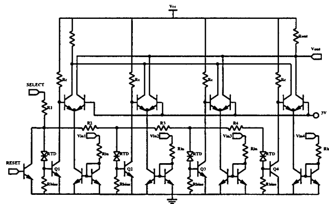
Figure 2: 4-input RTD multiplexer
