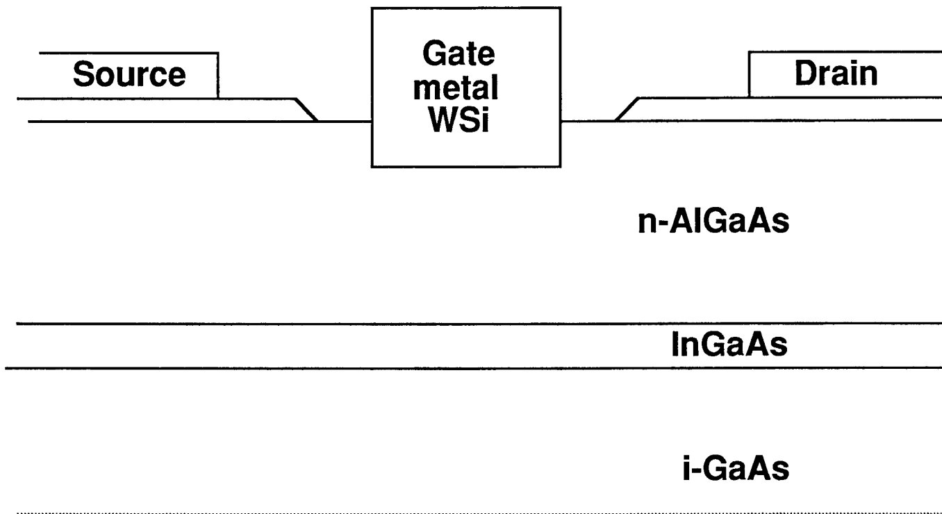
Fig. 1: HFET structure.
