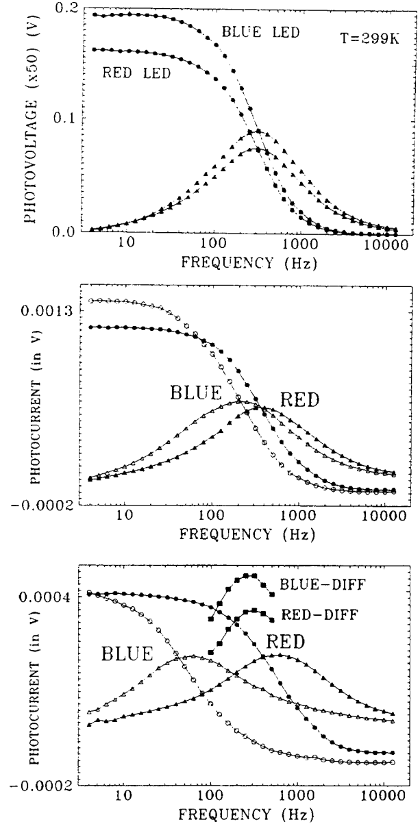
Figure 4. a) Photovoltage signals at the semitransparent gate under the two light sources described in the text. b) and c) Corresponding photocurrent signals (see text).
