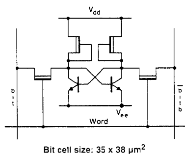
Figure 14. Schematic and microphotograph of BiFET memory cell.
