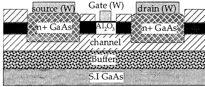
Fig.1 Schematic diagram of GaAs MISFET
