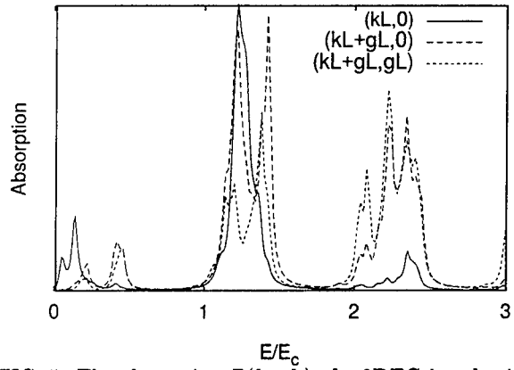
FIG. 5. The absorption P(\hbar\omega, \mathbf{k}) of a 2DEG in a lattice of antidots for three choices of the wave vector \mathbf{k} : \mathbf{k}L = (0.2, 0) , \mathbf{k}L = (0.2 + g_1L, 0) , and \mathbf{k}L = (0.2 + g_1L, g_2L) . E_c = \hbar\omega_c . Other parameters are as in Fig. 1.
