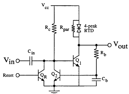
Figure 3: Four-valued down counter
