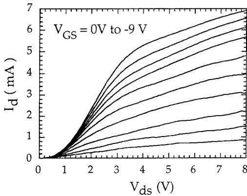
Fig.2 : I-V Characteristics of GaAs MISFET before hydrogenation
