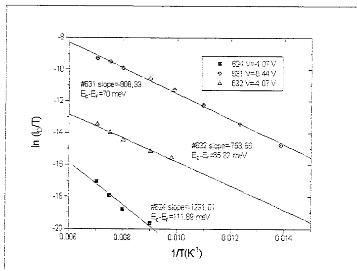
Fig 6. Dark current vs. temperature
