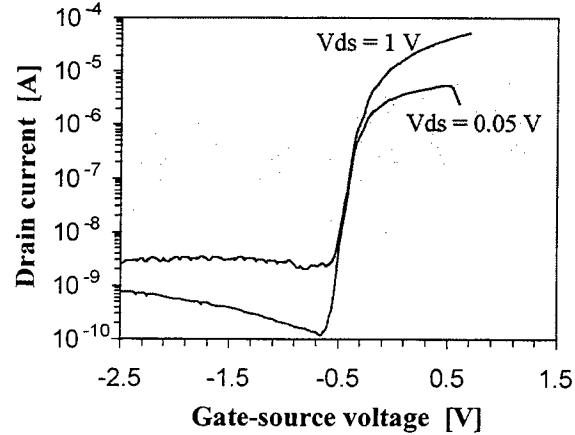
Fig. 4. Measured drain-current versus gate-source voltage characteristics of the same device as in Fig. 3.
