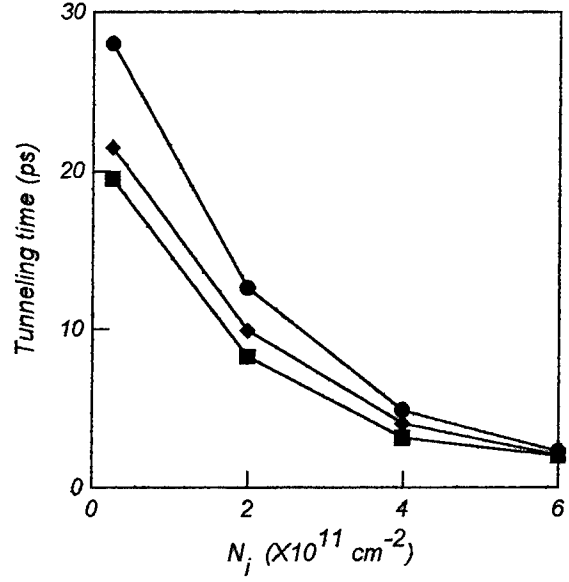
FIG. 4. Hole lifetimes vs N_i at different applied electric fields. Circles: F=1 kV/cm. Diamonds: F=5 kV/cm. Squares: F=10 kV/cm.
