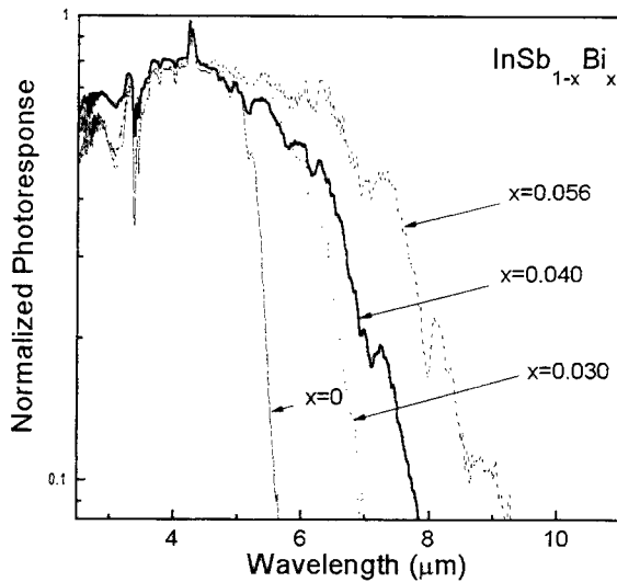
Figure 13. Normalized photoresponse of InSb 1-x Bi x alloys for various Sb compositions.
