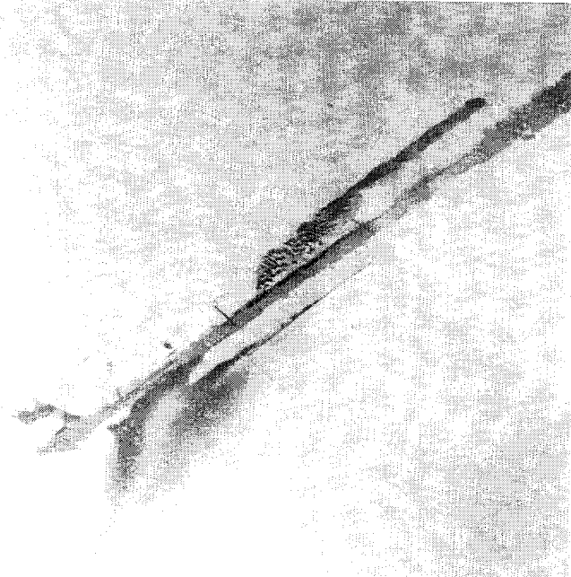
Figure E23. Tracer motion after a prototype equivalent of 2 hr 30 min under navigation wave N1 and spring peak flood water level and flow, full length weir opening
