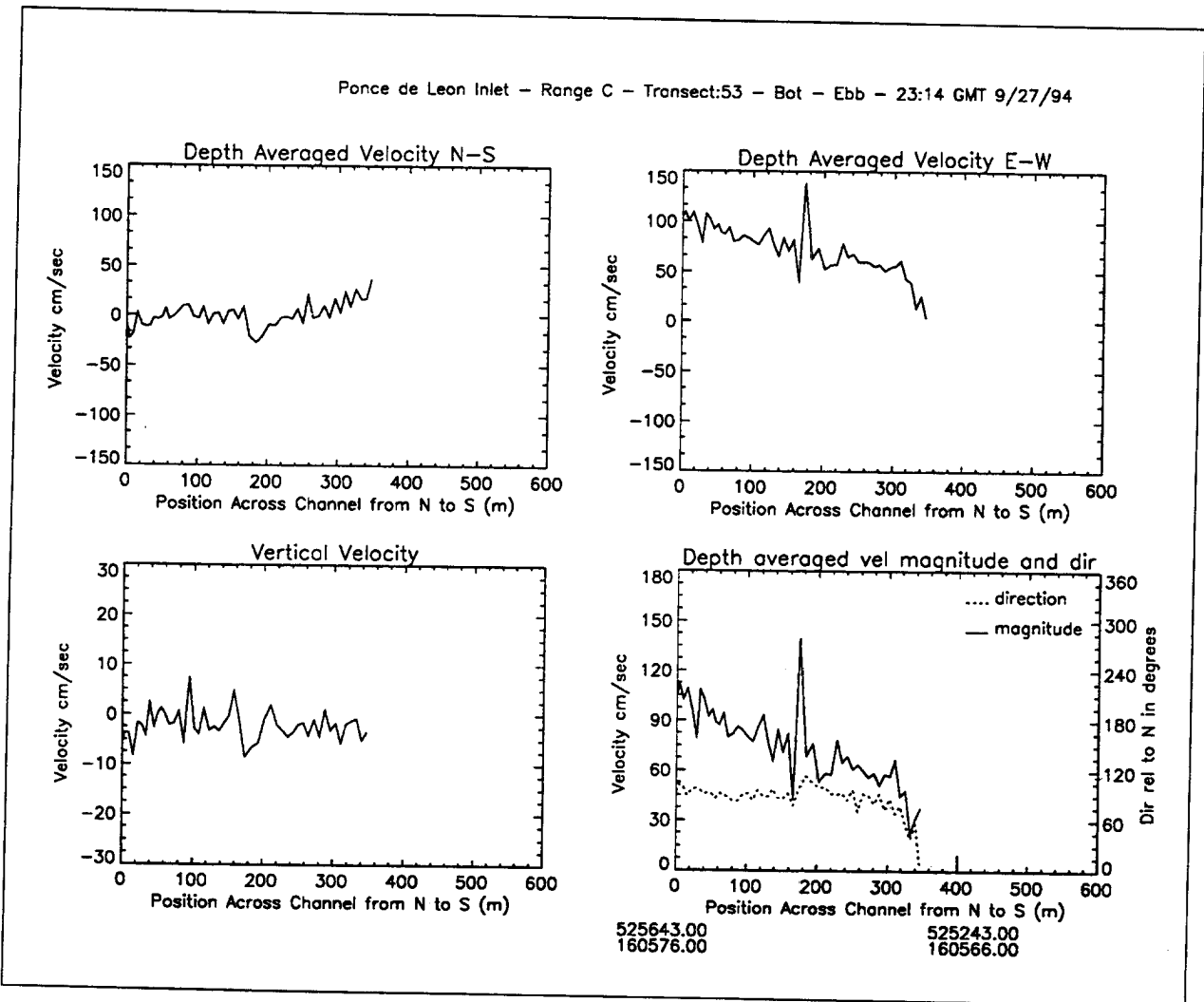
Figure 5. Example of depth-averaged magnitude and direction
