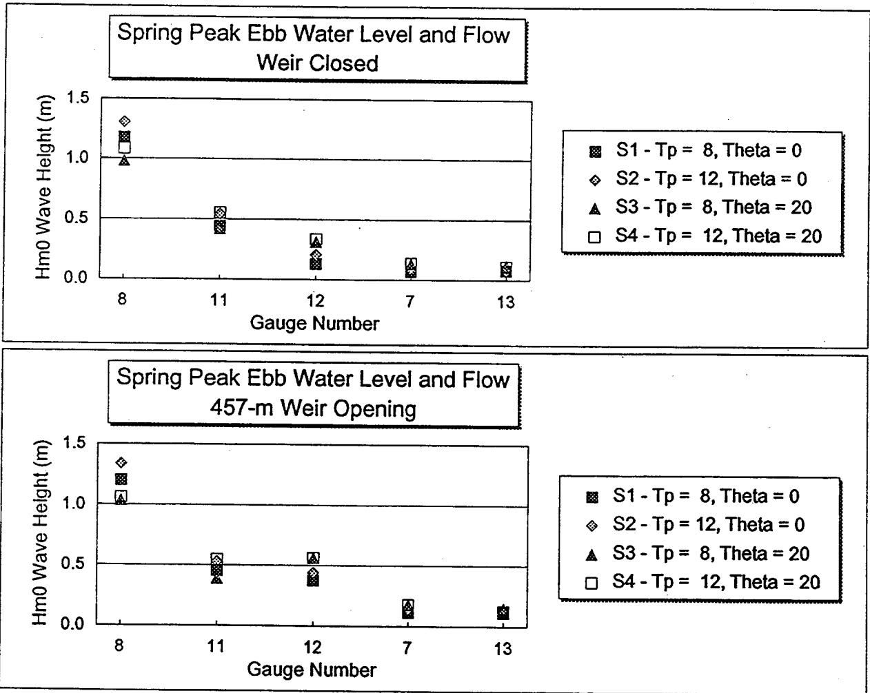
Figure 25. Wave attenuation with wave propagation down inlet channel for spring peak ebb water level for the weir closed and the 457-m (1,500-ft) weir opening
