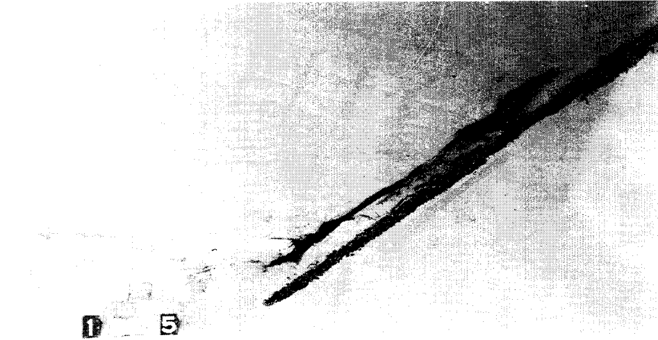
Figure E35. Tracer motion after a prototype equivalent of 2 hr 30 min under navigation wave N1 and spring peak ebb water level and flow, 152-m (500-ft) weir opening
