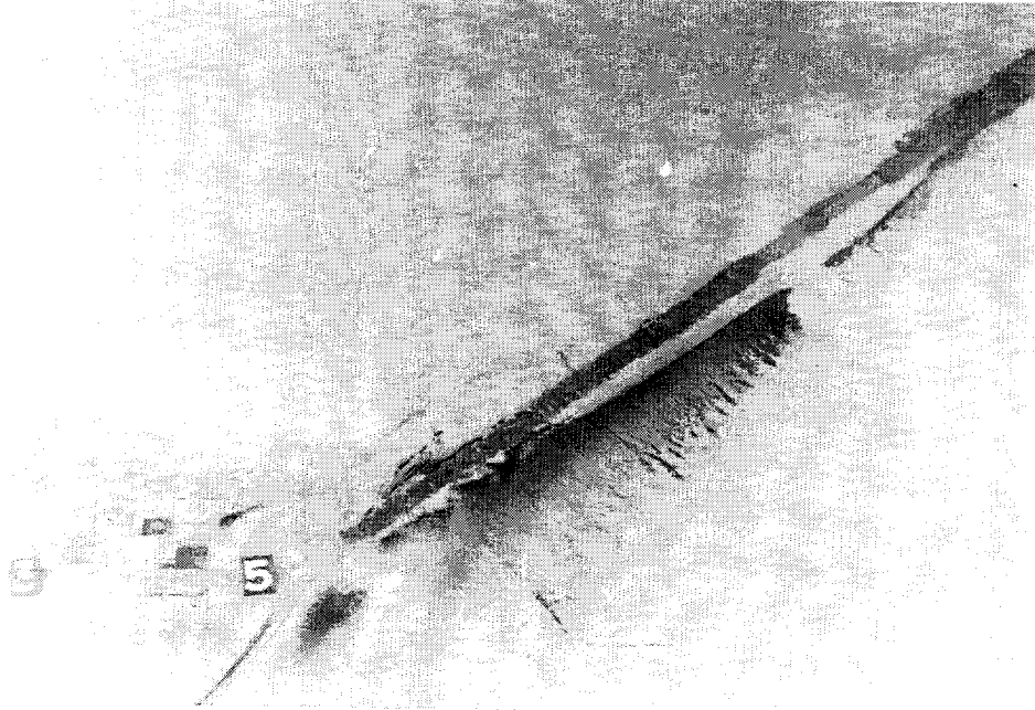
Figure E41. Tracer motion after a prototype equivalent of 2 hr 30 min under 1-year storm event and spring peak flood storm water level and flow. 152-m (500-ft) weir opening
