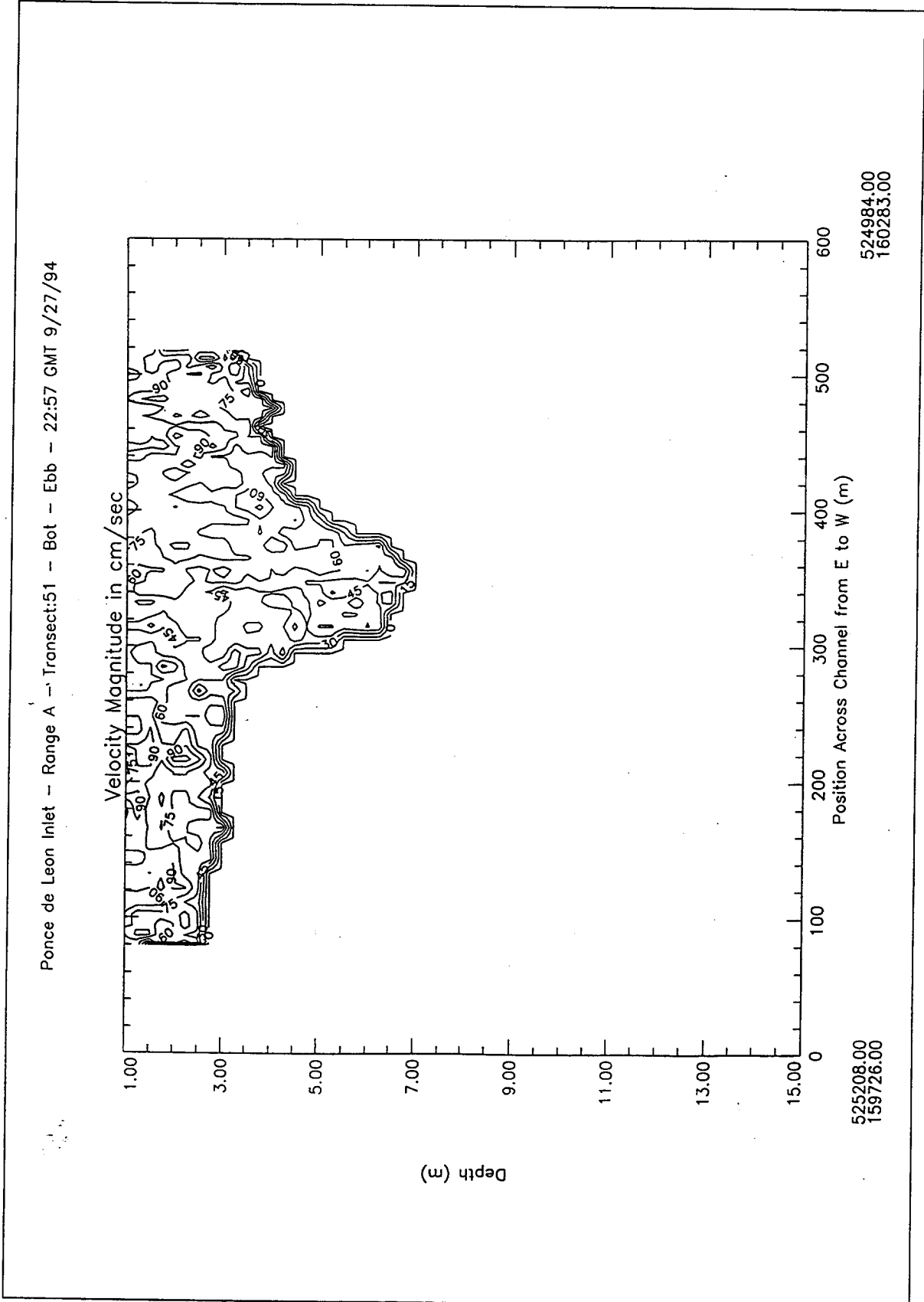
Figure B75. Contour plot of water magnitudes at peak ebb conditions, Range A, September
