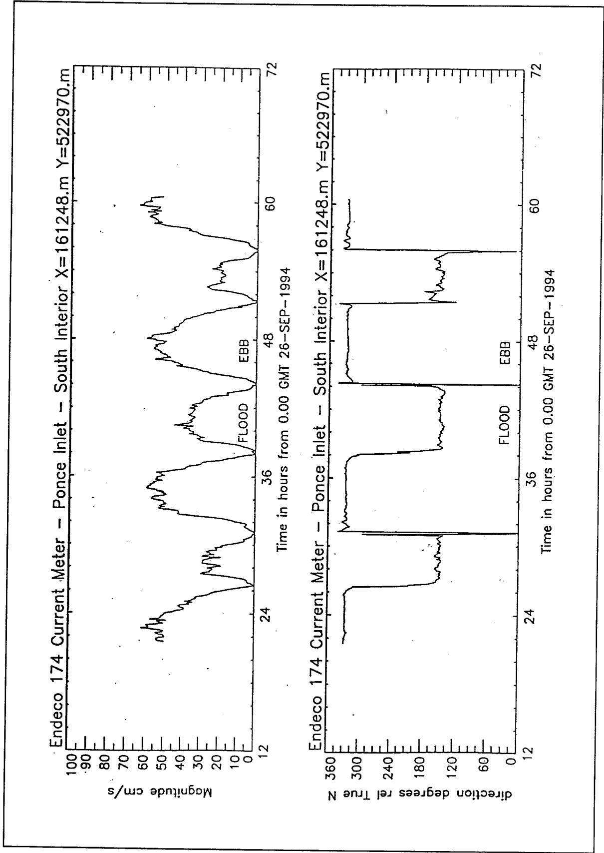
Figure C3. Current measurements at South Interior Site for September deployment
