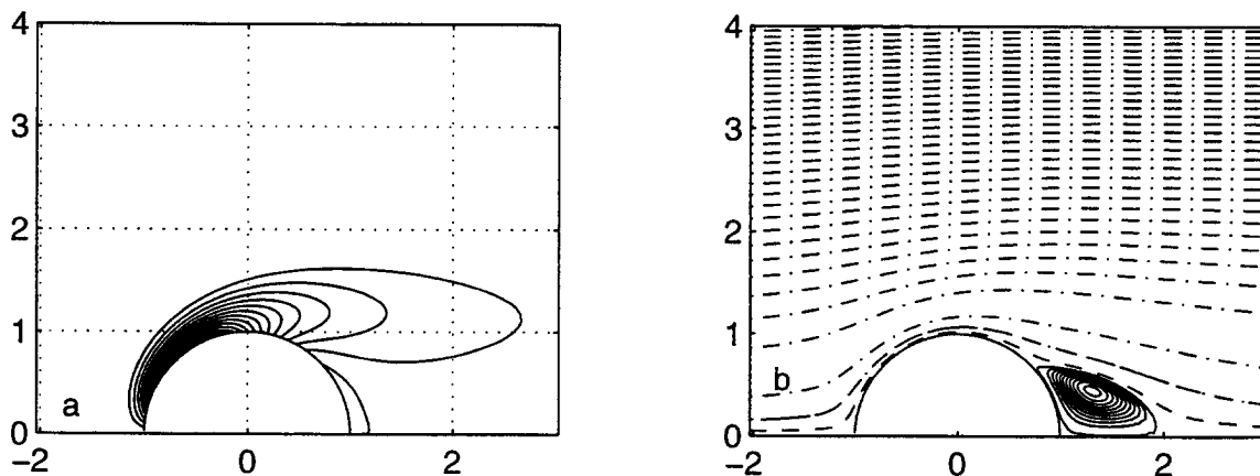
Figure 6. (a) Constant vorticity contours for Re = 56.5 \Delta\omega = 0.3 (b) Streamline contours \Delta\psi = 0.005 for '----', \Delta\psi = 0.15 for '-.-.-.-', \Delta\psi = 0.0003 for the separation region.
