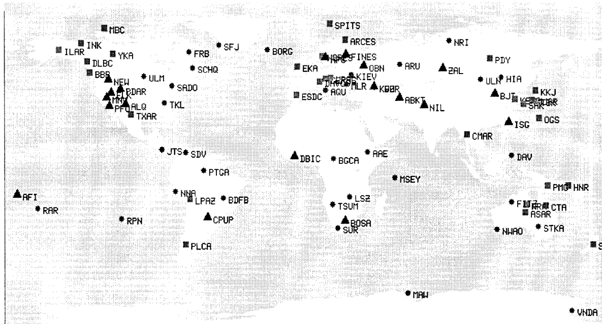
Figure 3. Locations of Primary and Auxiliary stations. Green squares: at least 20 regional events with at least one discriminant with SNR > 2.0; Blue triangles: at least 20 regional events with at least one discriminant with SNR > 1.5; Red circles: less than 20 regional events.
