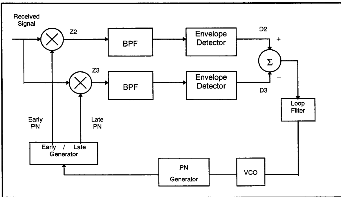
Figure 16. Delay Lock-Loop with Half-Chip-Delayed Correlator [Ref. 1]
