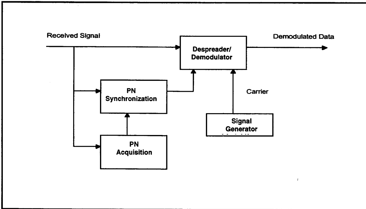
Figure 2. Demodulator Functional Block Diagram [Ref. 3]
