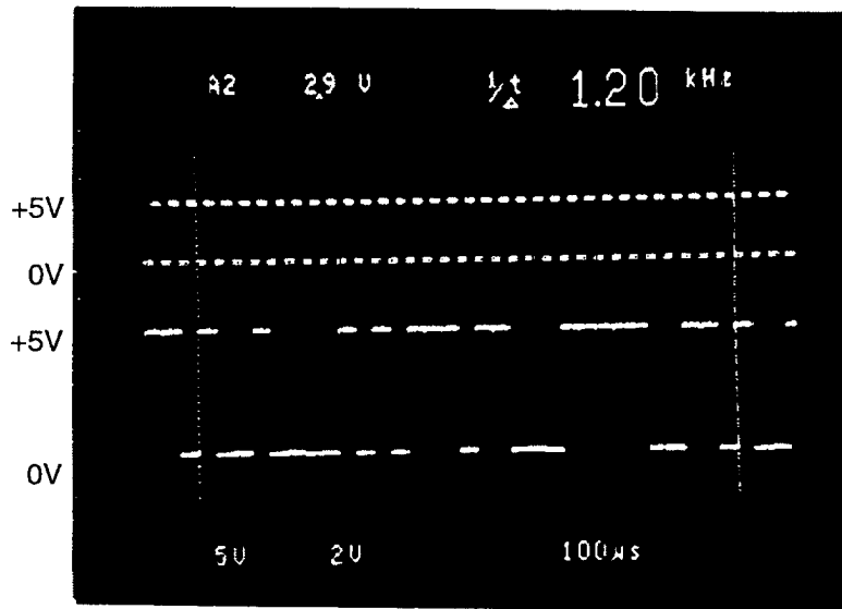
Figure 5. Top: Clock (37.2 kHz) Bottom: PN Sequence (Gold Sequence)
