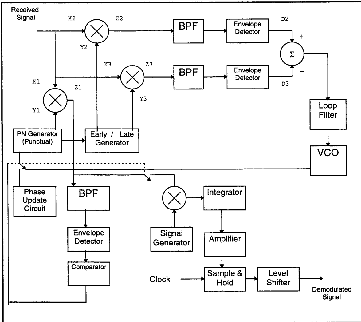
Figure 6. The Functional Block Diagram of the Demodulator
