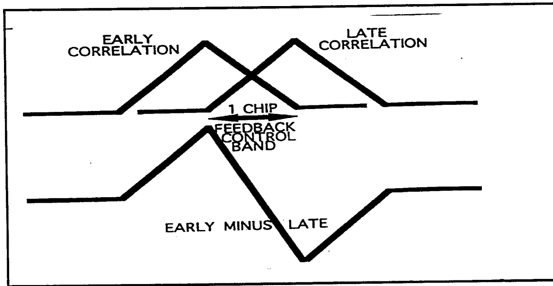
Figure 19. Ideal Early Minus Late Correlation Signal
