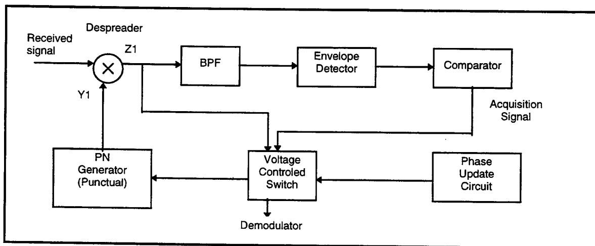
Figure 11. The Block Diagram of the Acquisition Circuit
