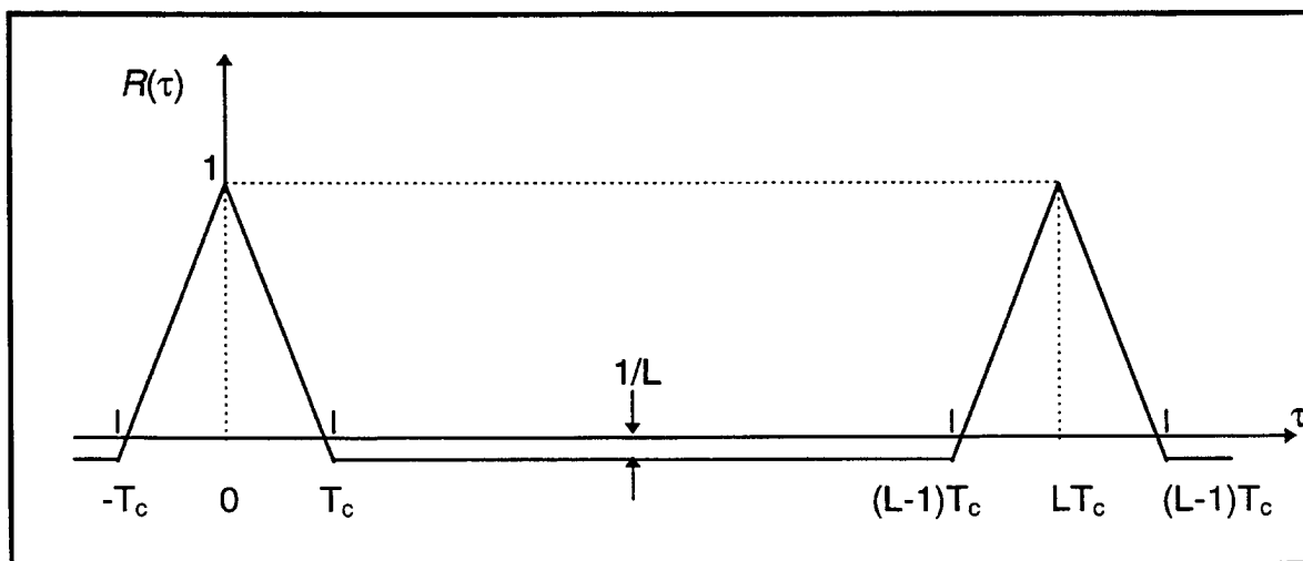
Figure 17. Ideal Correlation Triangle [Ref. 4]
