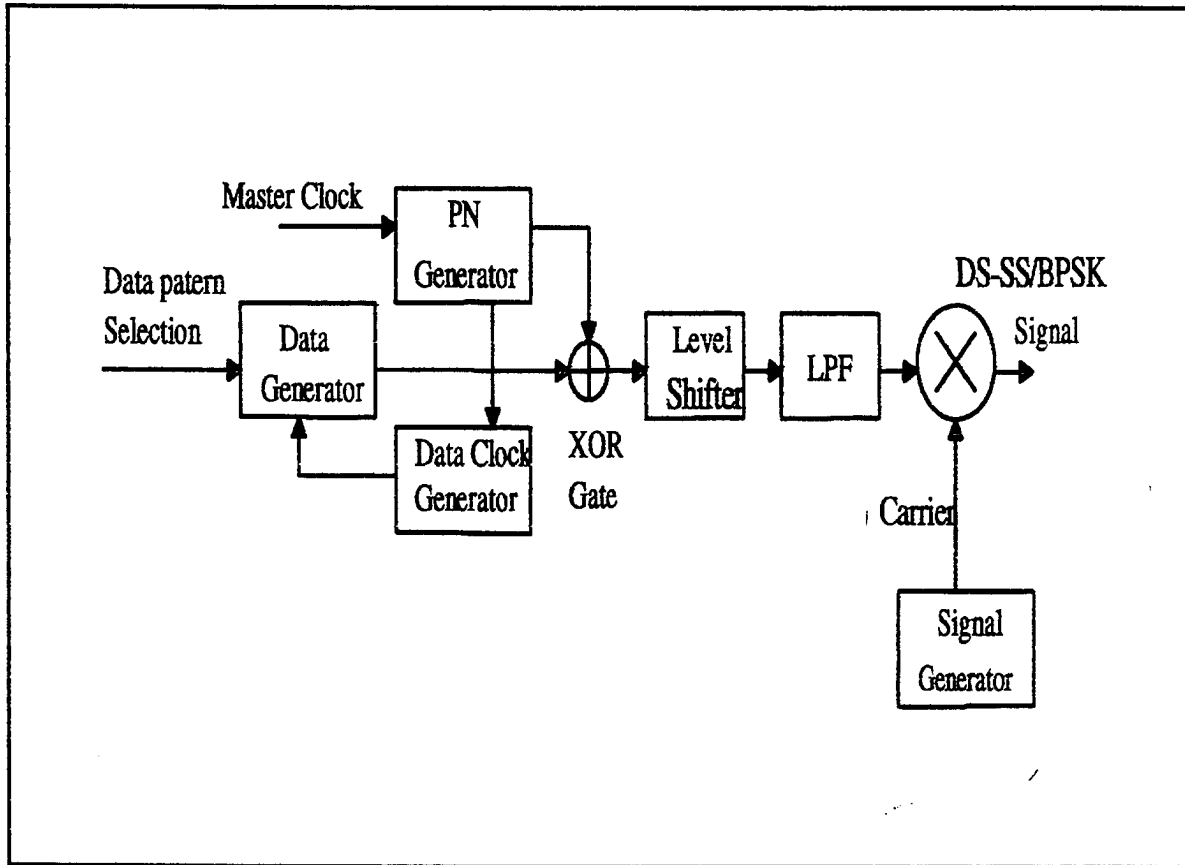
Figure A.1. The Modulator Functional Block Diagram.
