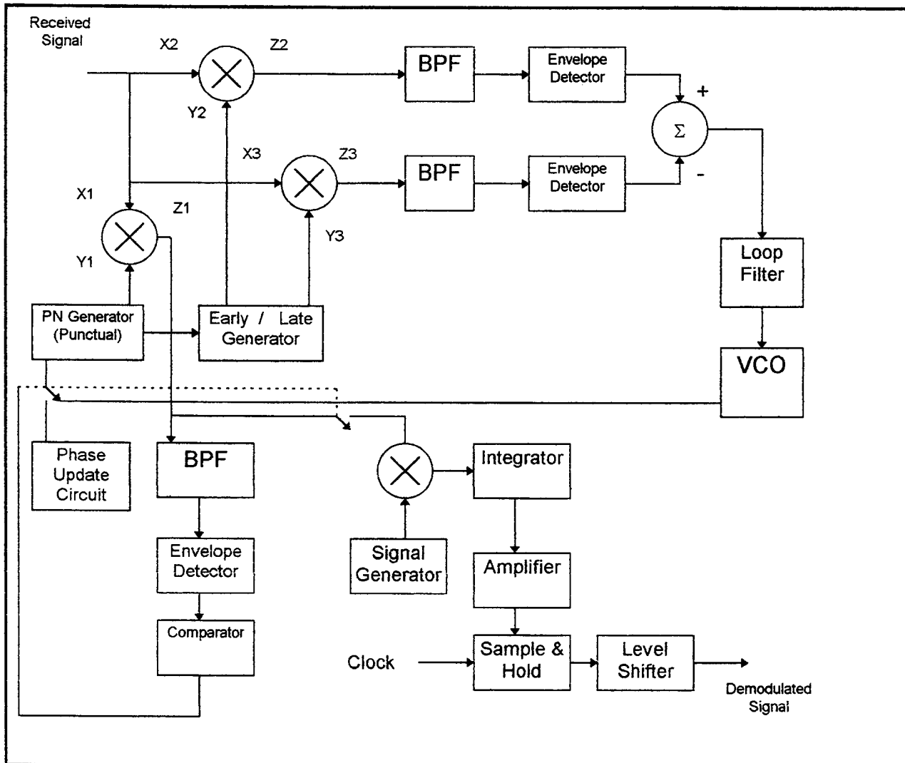
Figure A.2. The Functional Block Diagram of the Demodulator.
