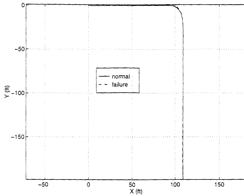
Figure 3.25 Increased r Sensor Noise (Position Plot).
