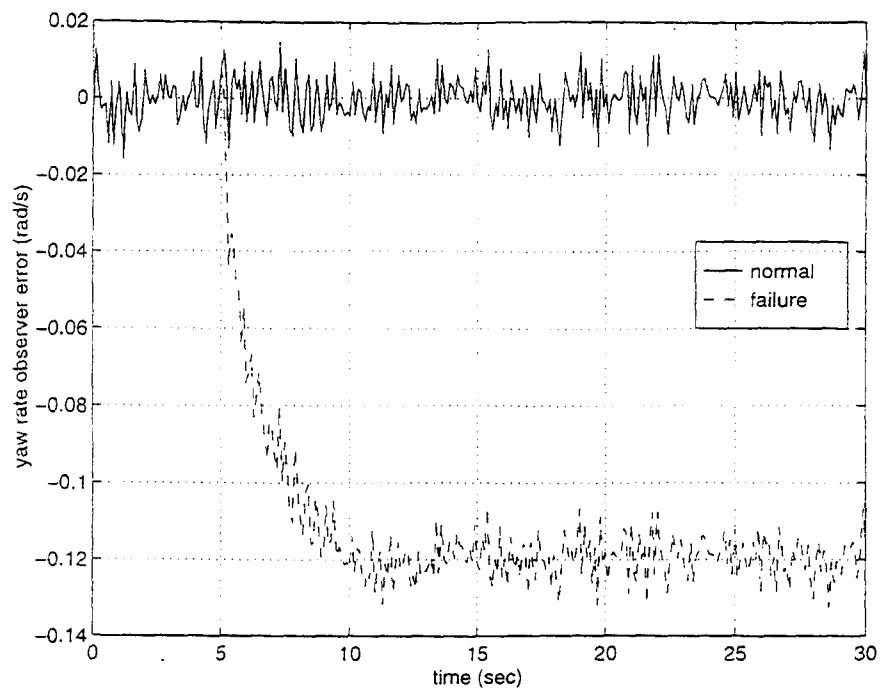
Figure 3.17 Hard Rudder ( e_{\dot{\psi}} vs time).
