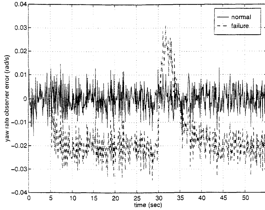
Figure 3.12 Stuck Rudder ( e_{or} vs time).
