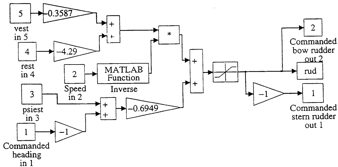
Figure 2.5 PD Controller Block.
