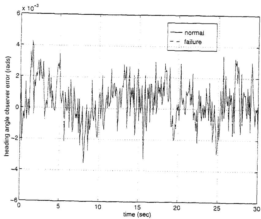
Figure 3.9 Stroke Limited Rudder ( e_{\psi} vs time).
