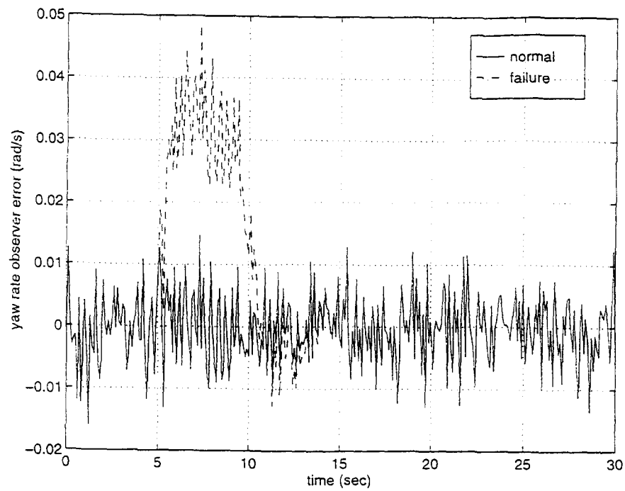
Figure 3.8 Stroke Limited Rudder ( e_{\dot{\psi}} vs time).
