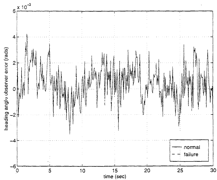
Figure 3.18 Hard Rudder ( e_{\psi} vs time).
