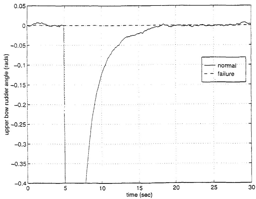
Figure 3.7 Loose Rudder ( \delta_{wrb} vs time).
