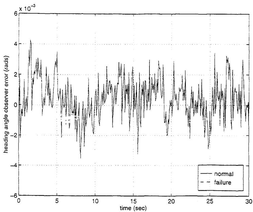
Figure 3.5 Loose Rudder ( e_{o\psi} vs time).
