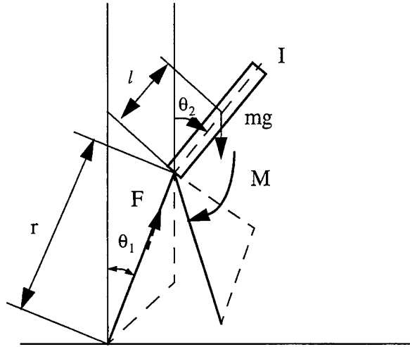
Figure 4: Single Rigid Body Model with Variable Length Massless Supporting Legs [GUBI74]
