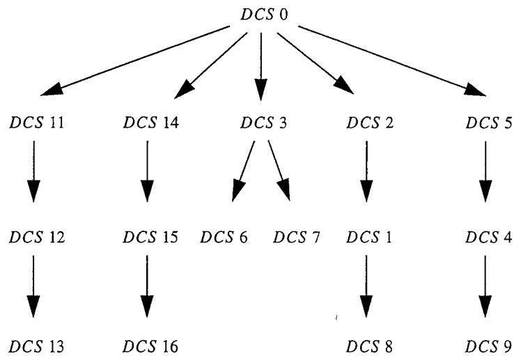
Figure 15: Dynamic Coordinate System (DCS) Hierarchy Tree of Dynaman
