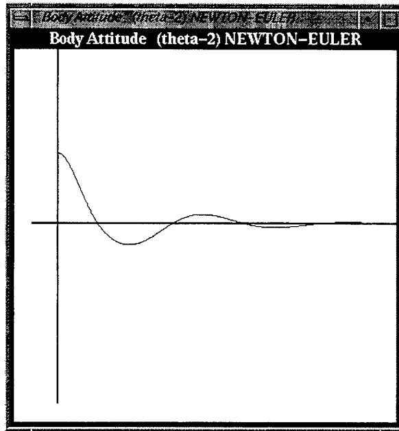
Figure 36: Body Attitude Time Response of the Two Link Inverted Pendulum (Newton-Euler)
