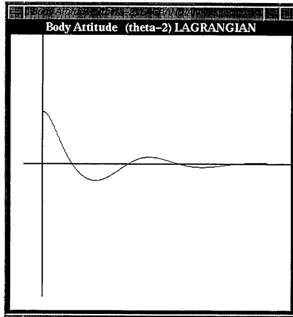
Figure 30: Body Attitude Response of the Two Link Inverted Pendulum (Lagrangian)
