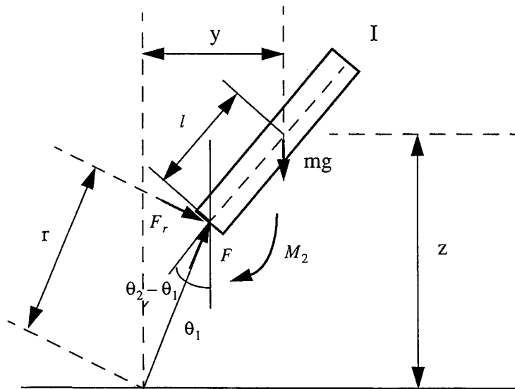
Figure 11: Free Body Diagram of The Body
