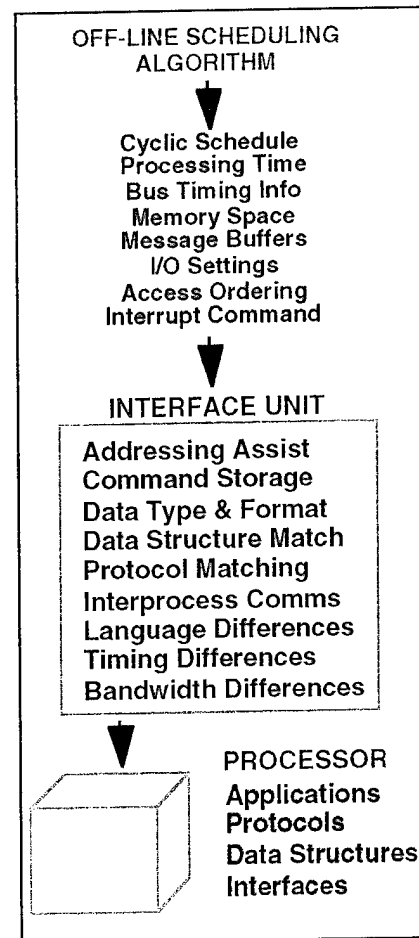
FIGURE 15. GENERAL MODEL FOR POST-FACTO INTEGRATION
