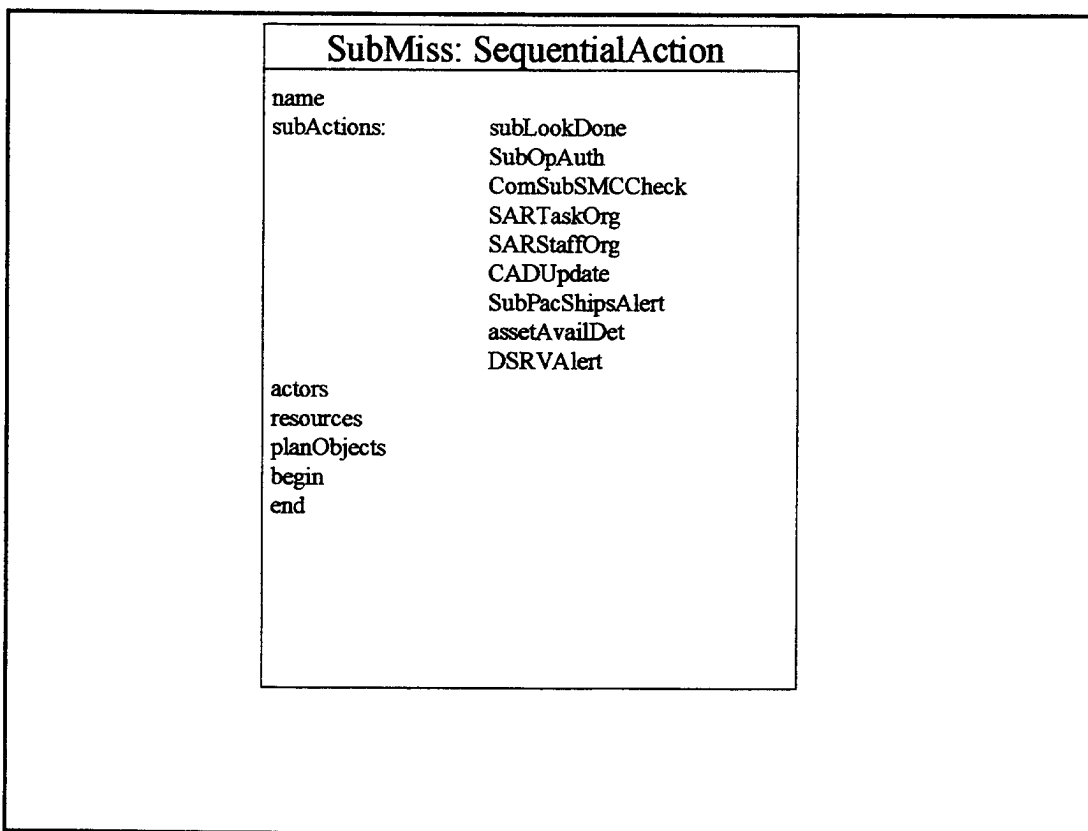
Figure 11. Action SUBMISS
