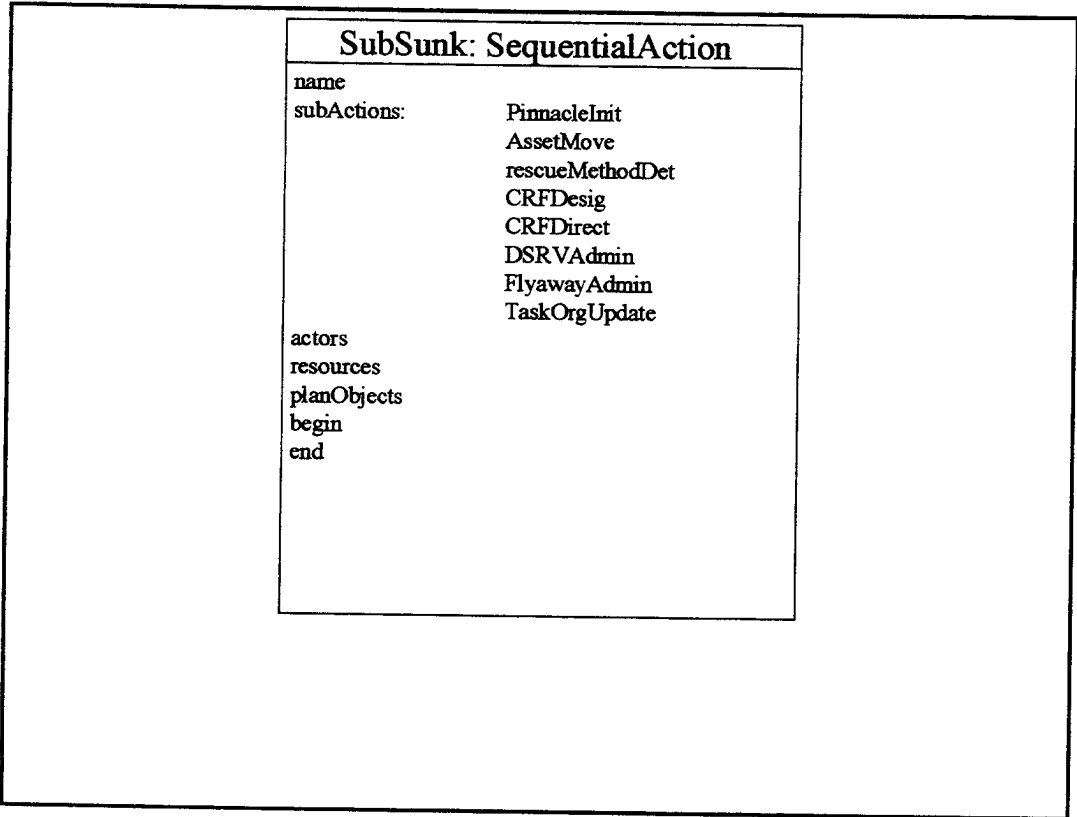
Figure 12. Action SUBSUNK
