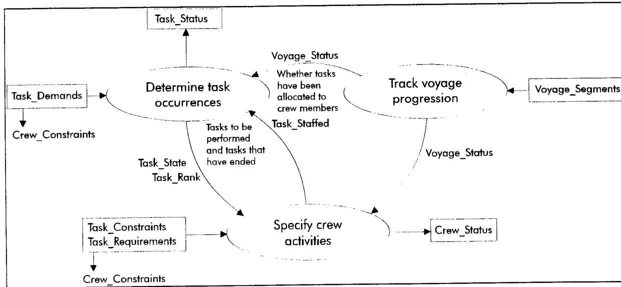
Figure 2. A data flow diagram of the basic simulation elements.
