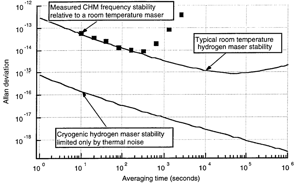
Fig. 1. Typical measured CHM and room temperature hydrogen maser frequency stabilities.
