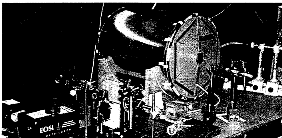
Fig. 2. Photograph of the first-generation double-bulb rubidium maser.
