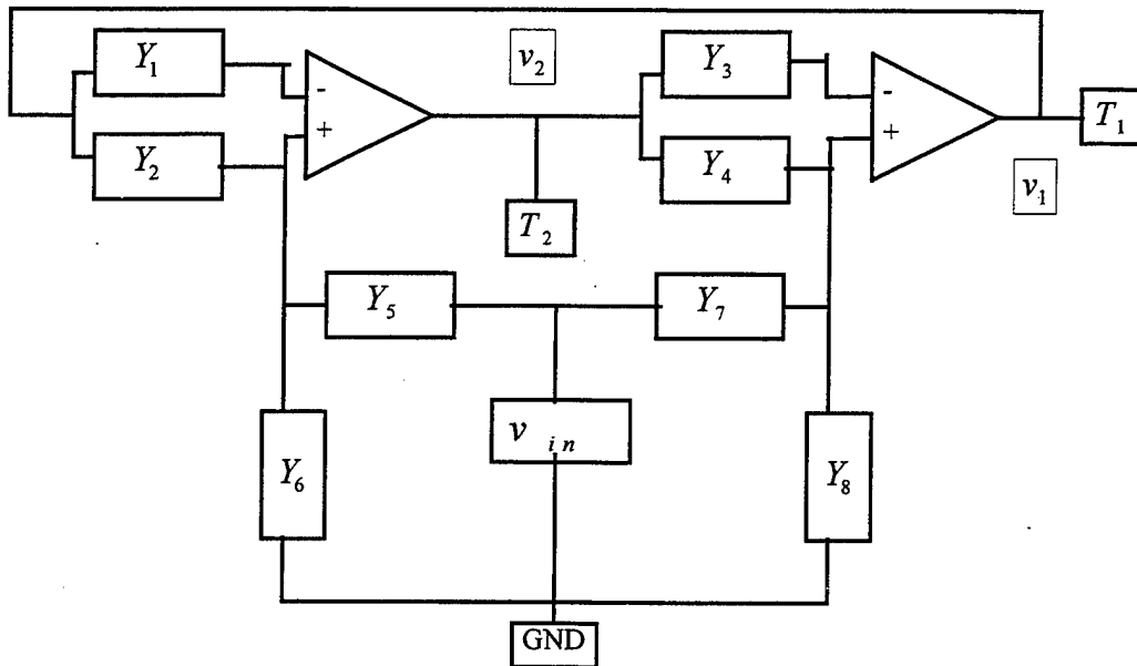
Figure 2.4 The General Immittance Converter Filter
