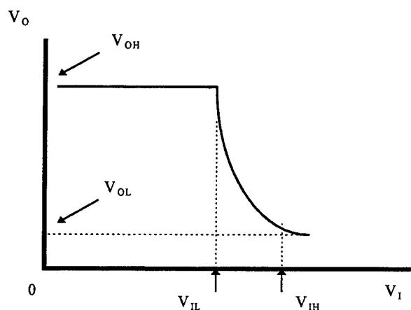
Figure 4.13 Transfer Characteristics of a DCFL Inverter
