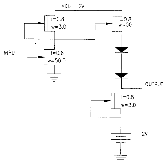
Figure 5.9 Clock Amplifier/Shifter
