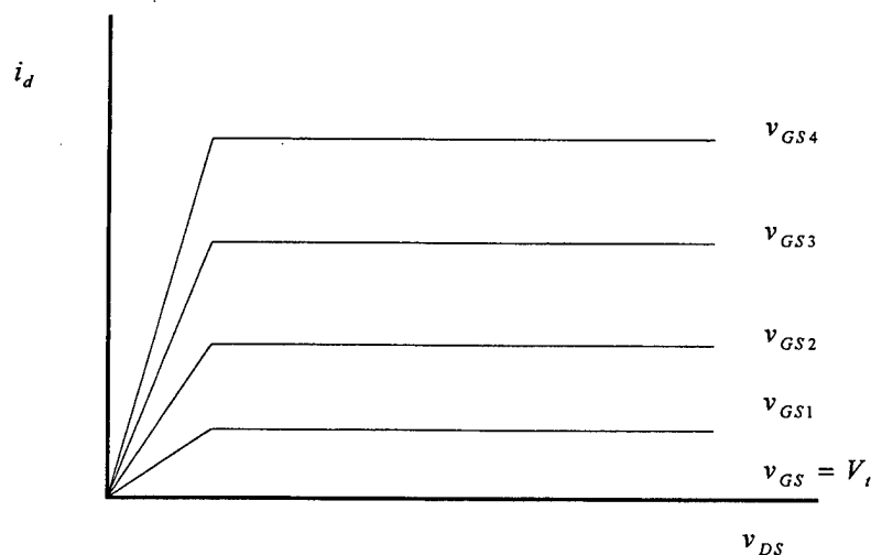
Figure 4.11 MESFET Drain Current vs Drain-to-Source Voltage
