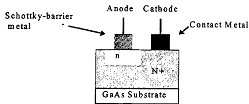
Figure 4.4 Cross Section of a GaAs SBD, Fisher (1995)
