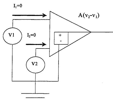
Figure 6.2 Equivalent Circuit for Ideal OPAMP, Sedra (1991)
