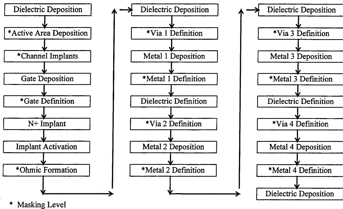
Figure 3.1 Vitesse H-GaAs III Process Sequence
