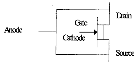
Figure 4.7 Symbolic Depiction of a MESFET as a Diode
