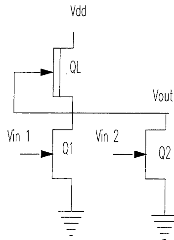
Figure 4.14 DCFL NOR Gate, Sedra (1991)
