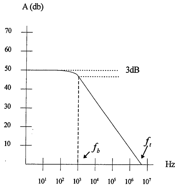
Figure 6.3 Frequency Response of an OPAMP
