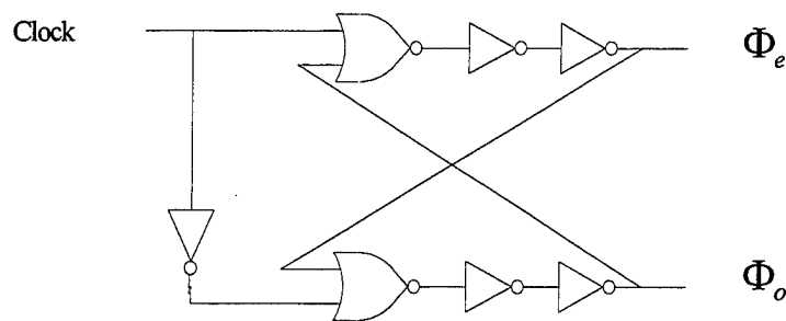
Figure 5.8 Two Phase Non-overlapping Clock, Schaumann (1990)
