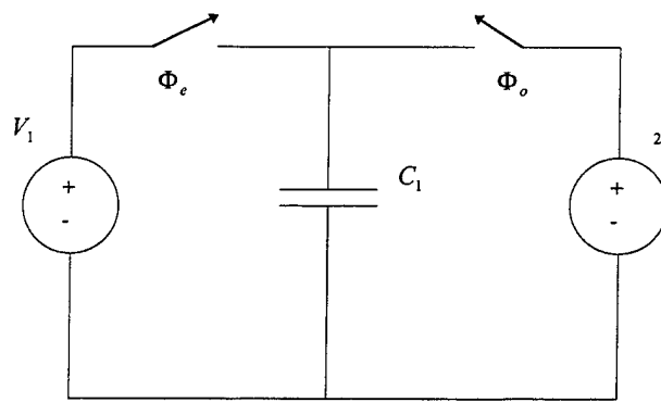
Figure 5.4 Parallel Switched Capacitor Network, Allen (1984)
