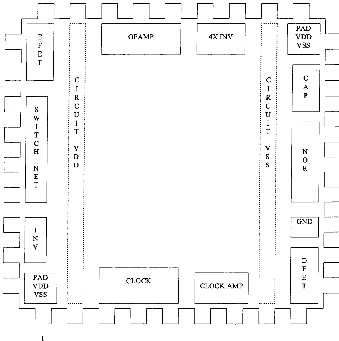
Figure 7.1 Project Chip Floor Plan
