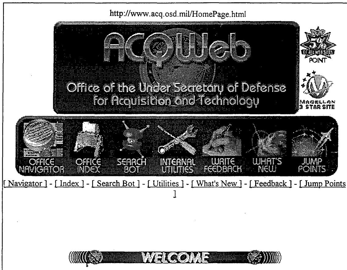
Figure 5.1. ACQWEB Homepage
