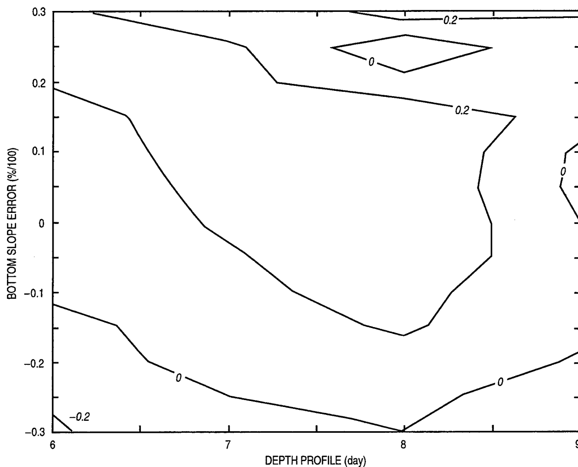
Fig. 10 — Contours of MSI fractional error for Depth Profile Error runs for 9 Oct using 9 Oct DELILAH data inputs and profiles d_{t,\gamma}
