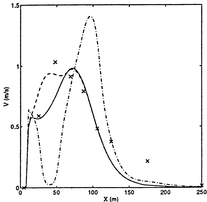
Figure 3. Predicted longshore currents compared with measured currents. The dashed line is the prediction including pressure gradient, rollers and mixing, the solid line is the prediction without the pressure gradient term, the dash-dotted line is the predicted current with no pressure gradient, roller or mixing, and observations are x marks. (from Reiners et al 1995)
