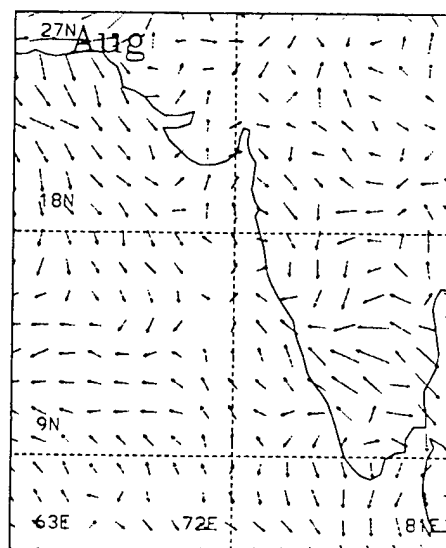
Figure 13. West India convergence diurnal components for May, June, July and August 1991. Phase and amplitude are represented in vector form based on a 24 hour clock with 12 midnight pointing north. All times are local time. Vector length indicates magnitude of convergence (-D850).
