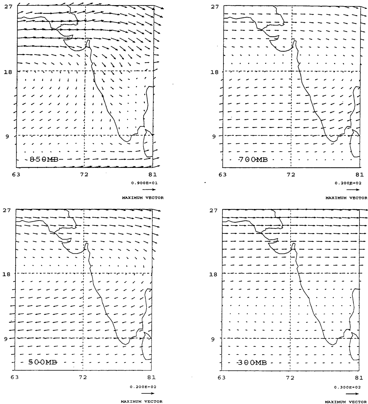
Figure 11. Monthly mean winds at 850, 700, 500 and 300 hPa for May 1991.
