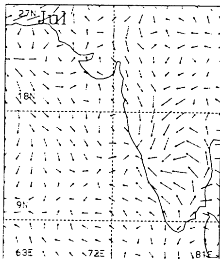
Figure 13. West India convergence diurnal components for May, June, July and August 1991. Phase and amplitude are represented in vector form based on a 24 hour clock with 12 midnight pointing north. All times are local time. Vector length indicates magnitude of convergence (-D850).
