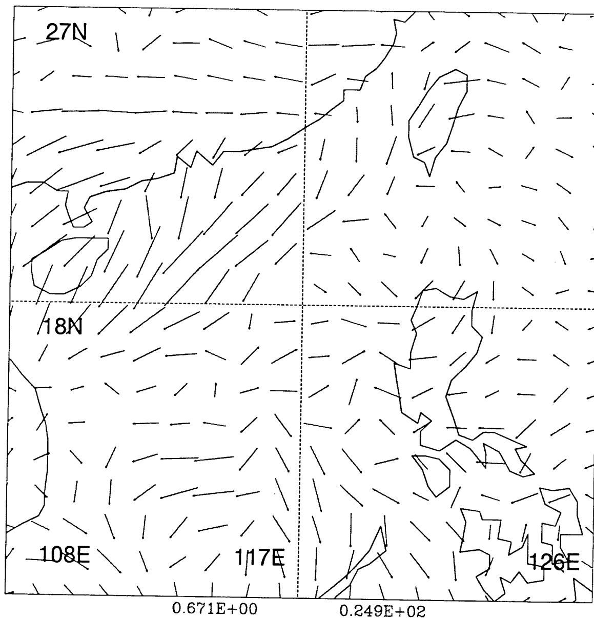
Figure 47. Northern South China Sea CI diurnal components for May, June, July and August 1991. Phase and amplitude are represented in vector form based on a 24 hour clock with 12 midnight pointing north. All times are local time. Vector length indicates magnitude of CI.
