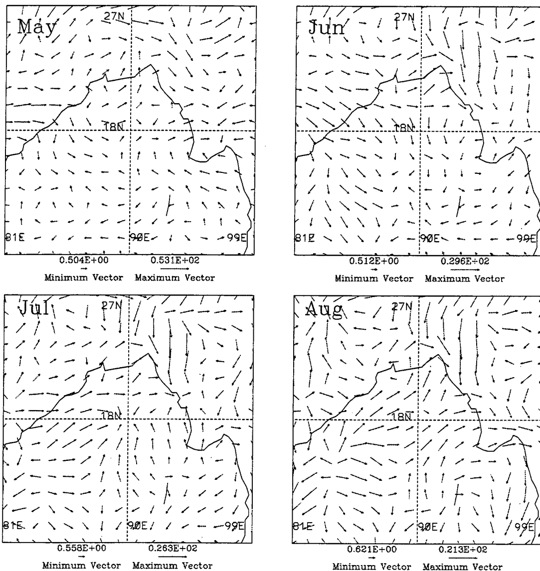
Figure 33. Bay of Bengal convergence diurnal components for May, June, July and August 1991. Phase and amplitude are represented in vector form based on a 24 hour clock with 12 midnight pointing north. All times are local time. Vector length indicates magnitude of convergence (-D850).
