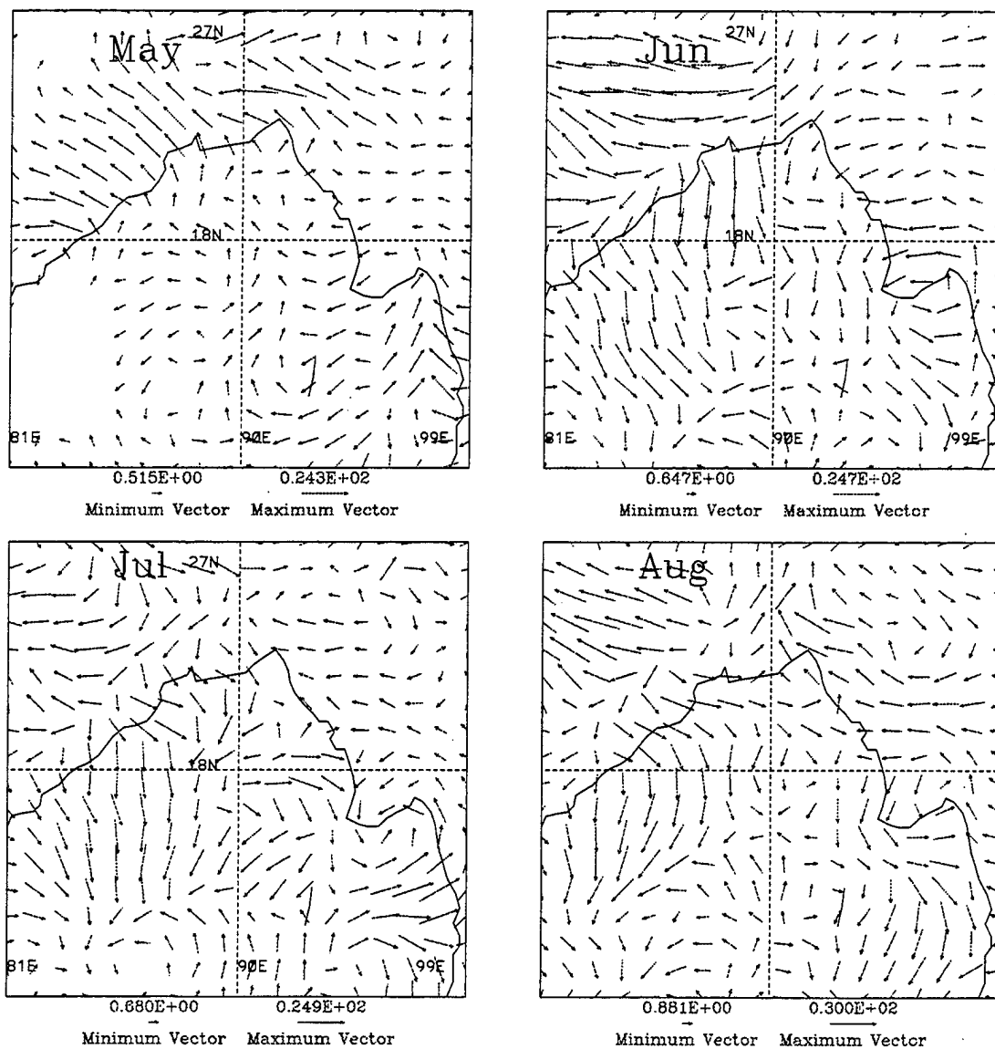
Figure 28. Bay of Bengal CI diurnal components for May, June, July and August 1991. Phase and amplitude are represented in vector form based on a 24 hour clock with 12 midnight pointing north. All times are local time. Vector length indicates magnitude of CI.
