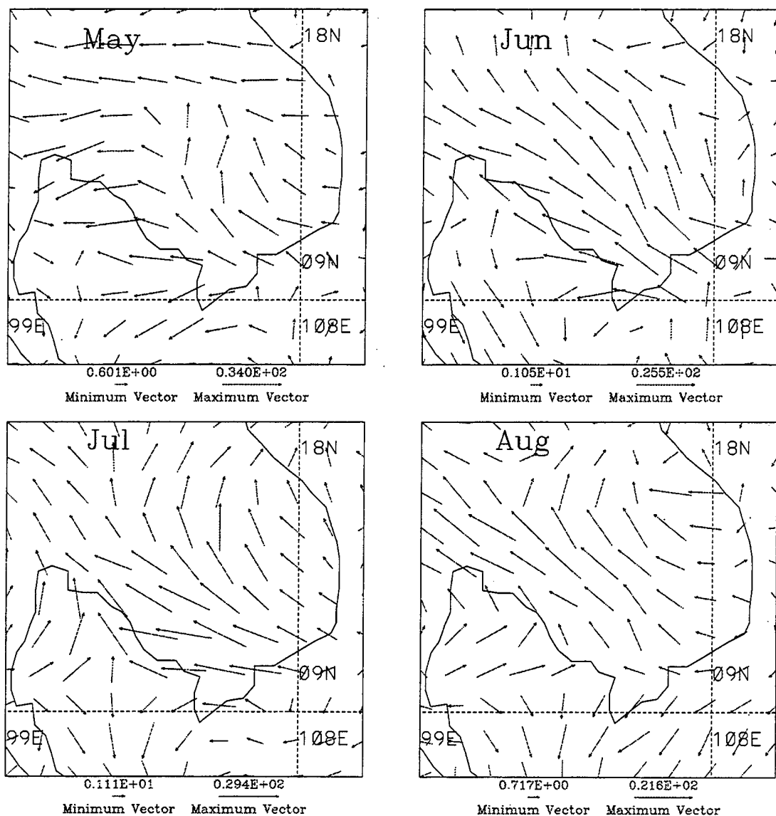
Figure 39. Indochina CI diurnal components for May, June, July and August 1991. Phase and amplitude are represented in vector form based on a 24 hour clock with 12 midnight pointing north. All times are local time. Vector length indicates magnitude of CI.
