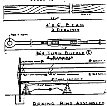
BOXING RING DETAIL SCALE: 1/2" = 1'-0"
