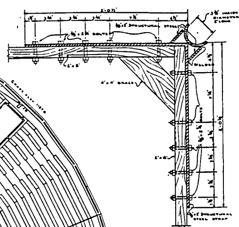
DETAIL OF STRUCTURAL STEEL STRAP SCALE: 1/2" = 1'-0"
