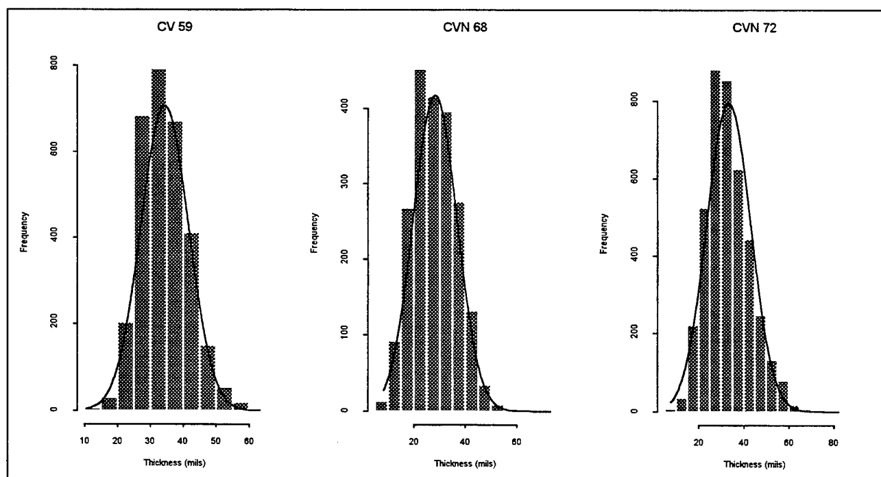
Figure 2. Normal density plots for three freshly applied coating systems.
