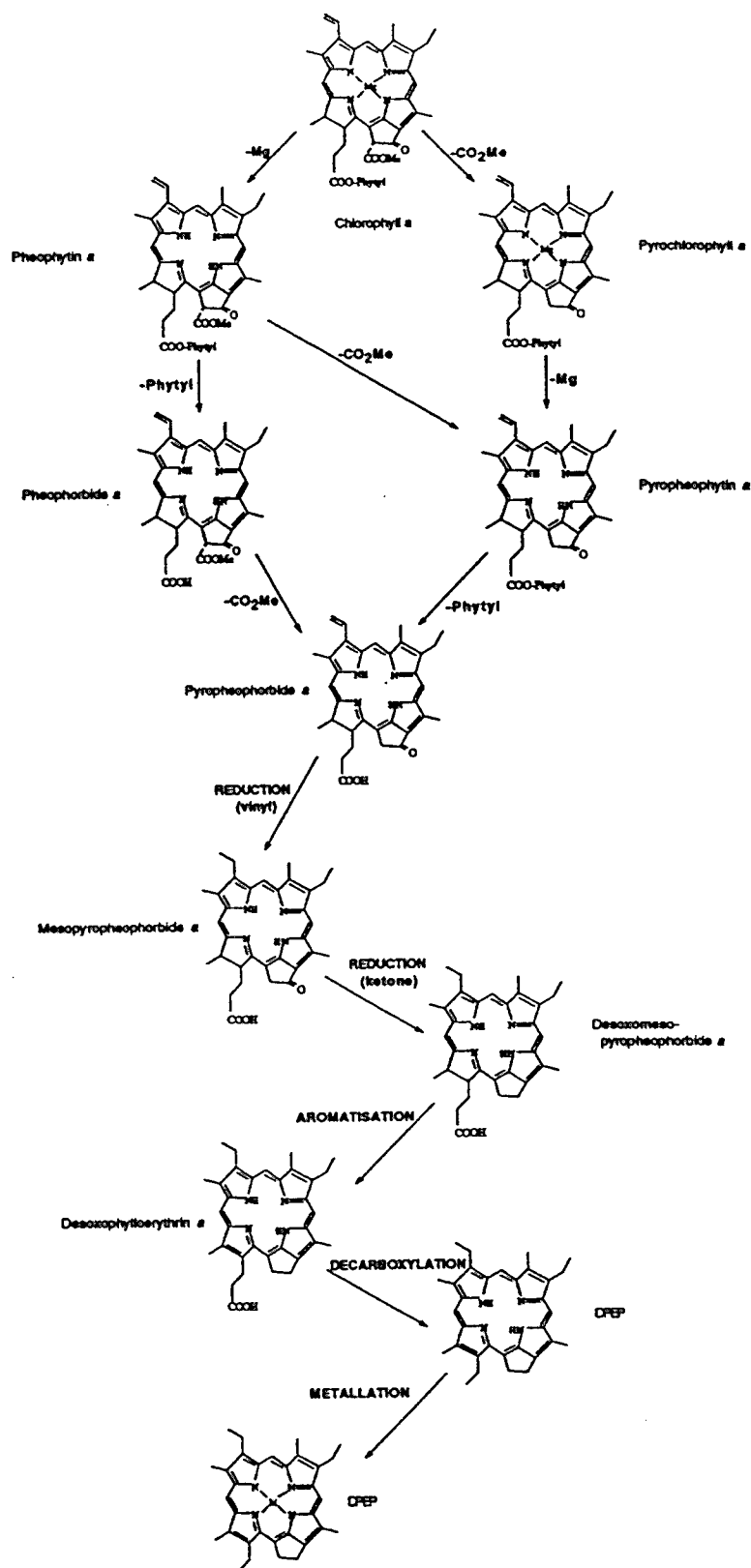
Figure 1.3: Possible transformation pathways for chlorophyll a to DPEP. First proposed by Treibs (1936). Figure adapted from Keely (1990) by Huseby (1996).
