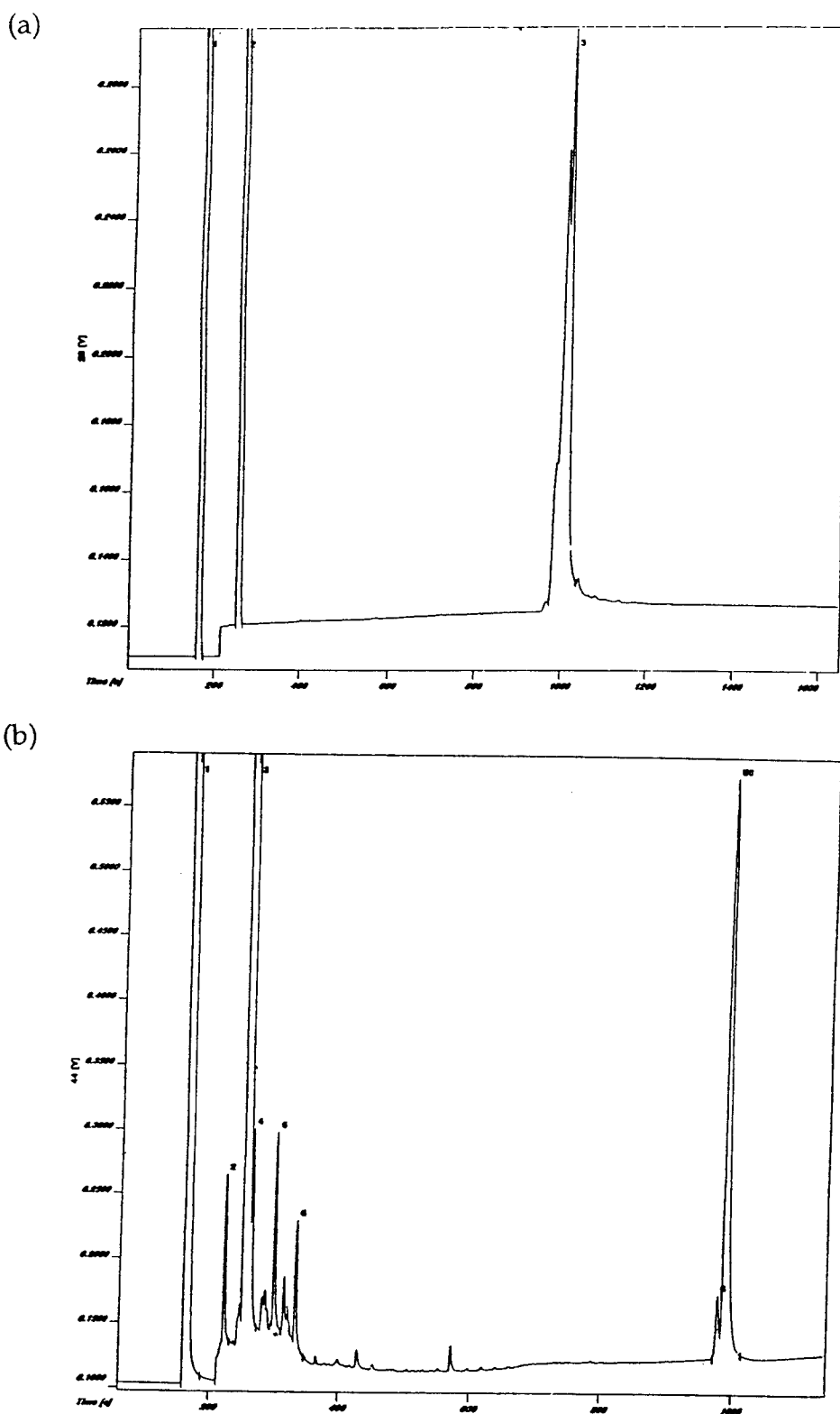
Figure 3.15: Chromatograms from irmGC-MS runs of derivatized 9MPPBDa. The results for \delta^{15}\text{N} ( ^{14}\text{N}_2 =mass 28) are shown in (a), while those for \delta^{13}\text{C} ( ^{12}\text{C}^{16}\text{O}_2 =mass 44) are shown in (b). The peak splitting in (a) resulted from overloading the GC column.
