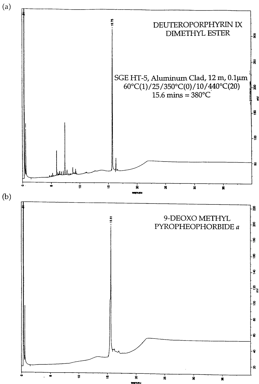
Figure 3.24: Gas chromatograms of (a) deuteroporphyrin IX dimethyl ester, and (b) 9-deoxo-methyl pyropheophorbide a .
