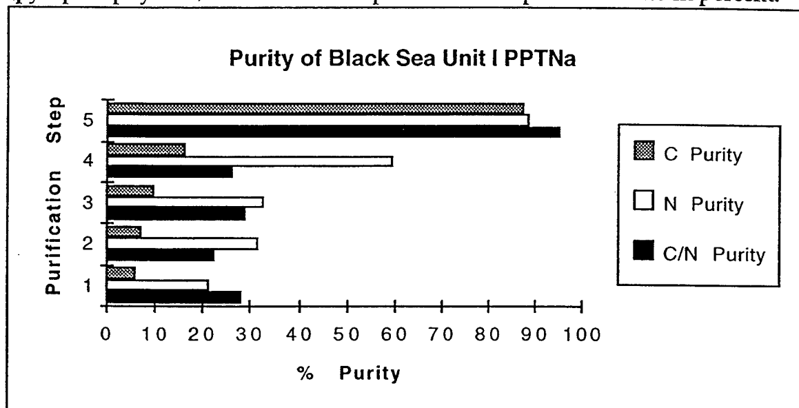
Figure 2.7: Purity of a Black Sea surficial sedimentary chlorin (pyropheophytin a ) after successive purification steps. Values are in percent.
