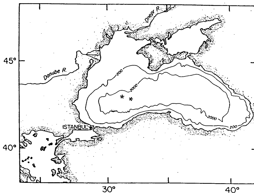
Figure 5.4: Map of the Black Sea showing sample locations.
