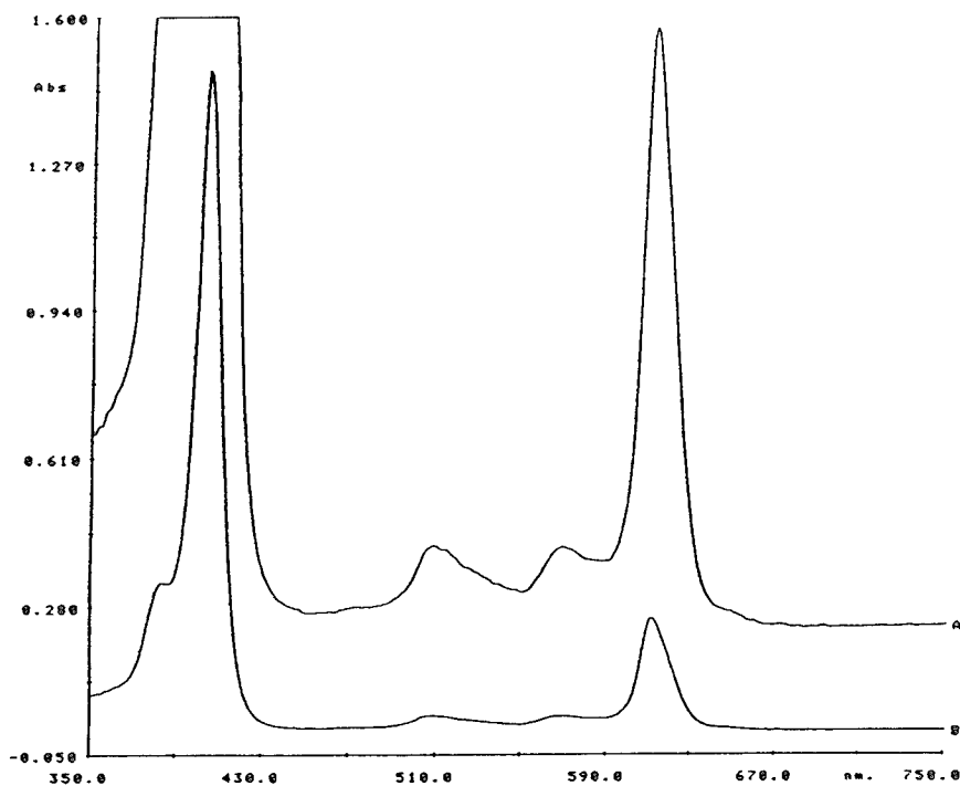
Figure 3.9: Visible spectrum of (9MPPBDa)Si(OTBDMS) 2 in hexane. Absorbance maxima are at 403, 508, 568, and 610 nm.
