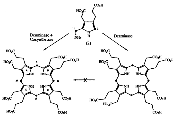
Figure 4.7: Condensation of 4 PBG molecules to form hydroxymethylbilane. Figure from Leeper (1991).
