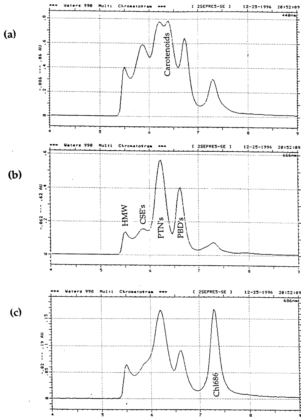
Figure 2.5: Size-exclusion chromatograms of a surface Peru margin sediment extract at (a) 440 nm, (b) 666 nm, and (c) 686 nm. The column was a Shodex GPC K-801 (8 mm I.D. x 300 mm length; Showa Denko K.K., Tokyo, Japan), the eluant was MeCl 2 , and the flow rate was 1.0 mL/min. Pigment abbreviations are as follows: HMW=high molecular weight chlorin, CSE=chlorin steryl esters, PTN=pheophytins, PBD=pheophorbides, and Chl686 is an unknown chlorin discussed in section 2.5.3.1.
