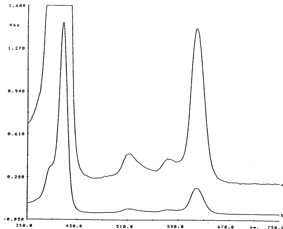
Figure 3.6: Visible spectrum of (9MPPBDa)Si(OH) 2 in MeCl 2 . Absorbance maxima are at 405, 511, 572, and 617 nm.
