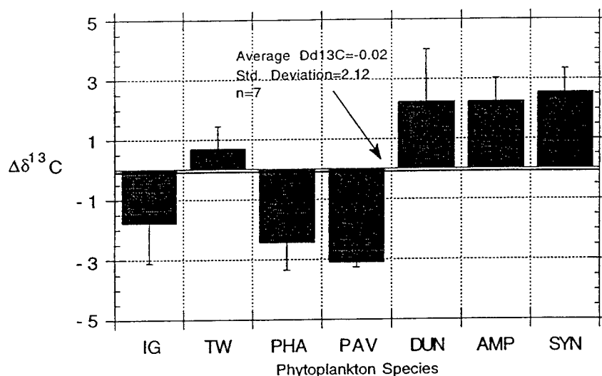
Figure 4.12: The carbon isotopic difference between chlorophyll and whole cells, \Delta\delta^{13}\text{C}_{\text{cell-Chl}a} , for 7 species of marine phytoplankton. See text for an explanation of error bars, and table 4.1 for species abbreviations.
