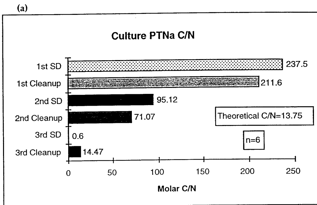
Figure 2.6: Purity of algal pheophytin a following each step of the procedure for the purification of particulate chlorins for isotopic analysis. Figure (a) shows the average C/N ratio of the products, (b) shows pheophytin a purity based upon the measured versus theoretical C/N ratio, and (c) and (d) show nitrogen and carbon purities of the pheophytin a , respectively. All values are averages of 6 cultures, and standard deviations (SD) are plotted. See text for an explanation of the purification steps.
