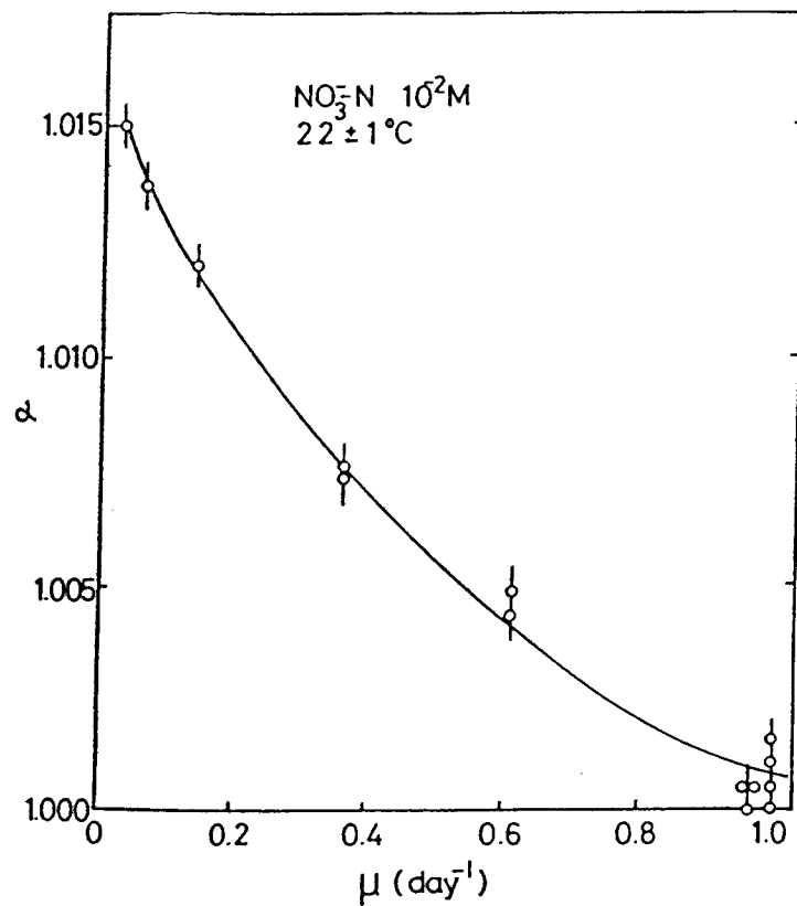
Figure 4.11: Relationship between nitrogen isotopic fractionation during nitrate assimilation and growth rate. The fractionation factor, \alpha , is plotted versus the growth rate constant, \mu . Figure from Wada and Hattori (1978).
