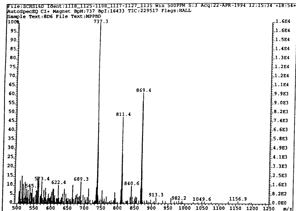
Figure 3.21: GC-CI + mass spectrum of compound eluting 19 seconds after (MPPBDa)Si(OTBDMS) 2 . The fragmentation pattern is virtually identical to that of the desired product (figure 3.20), yet each fragment is 32 mass units greater (see text for discussion).
