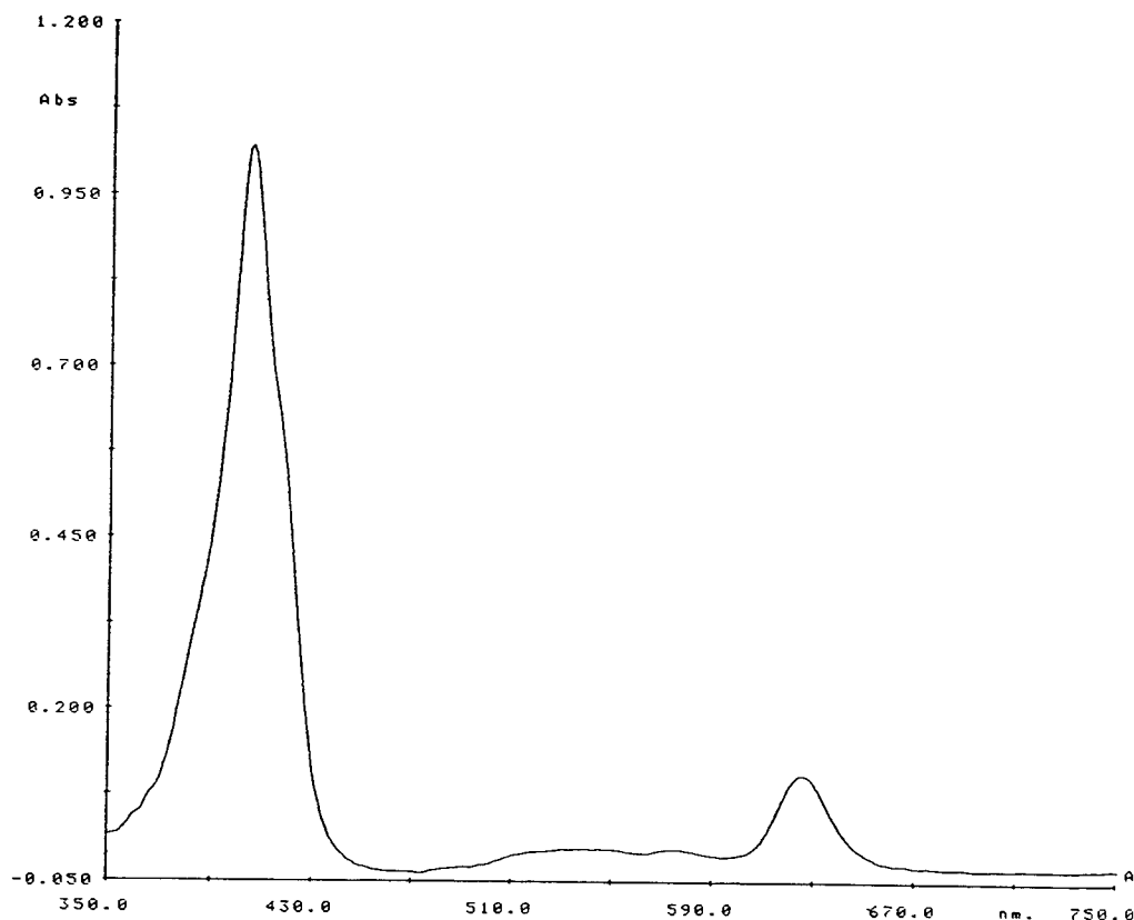
Figure 3.5: Visible spectrum of (9MPPBDa)SiCl 2 in MeOH. The red band migrated to 624 nm in the dichlorosilicon complex from 648 nm in the free-base .
