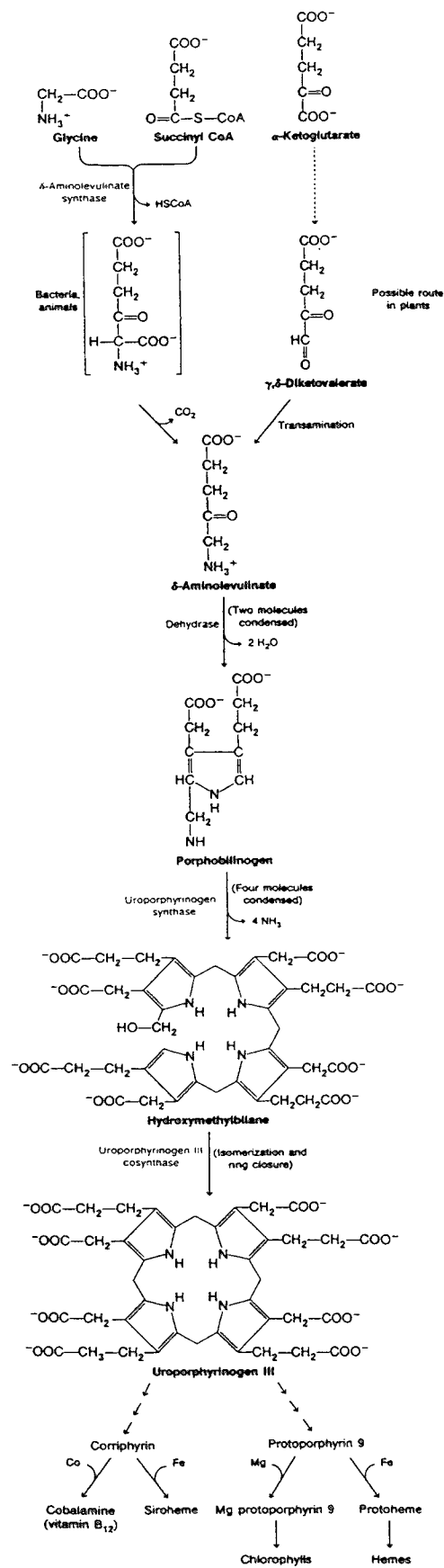
Figure 4.6: (continued). Figure from Zubay (1983).
