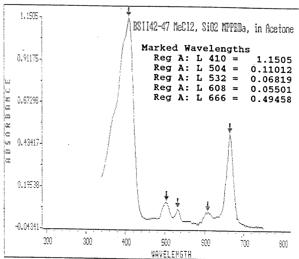
Figure 2.1: Visible spectra of (a) a whole sediment extract from Unit II of the Black Sea, and (b) the most abundant chlorin in that extract (e.g., MPPBDa) after purification according to procedures developed in this study.
