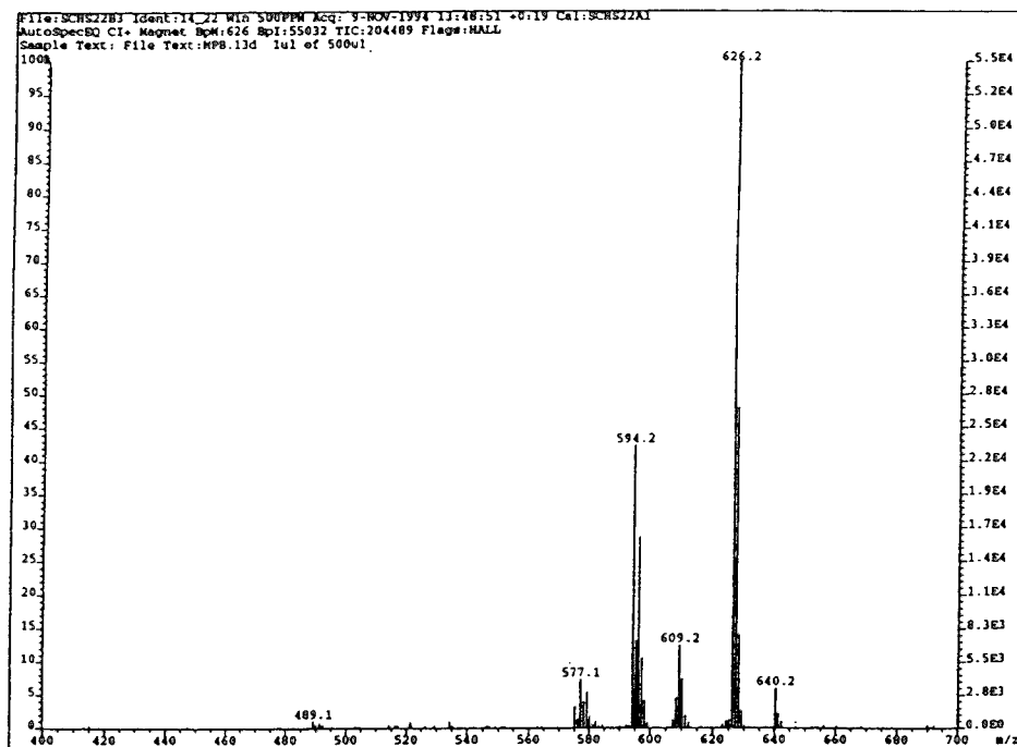
Figure 3.22: Methane CI-mass spectrum of (9MPPBDa)Si(OH) 2 (M/Z=594 (M, 40%)) showing the high abundance of the M+32 side-product (M/Z=626, 100%), corresponding to the addition of CH 4 O.
