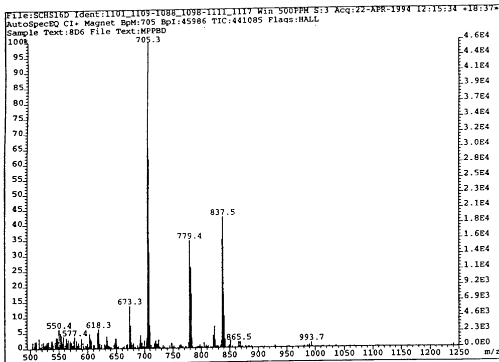
Figure 3.20: GC-CI + mass spectrum of (MPPBDa)Si(OTBDMS) 2 . The retention time of the derivative was 18:36 minutes.
