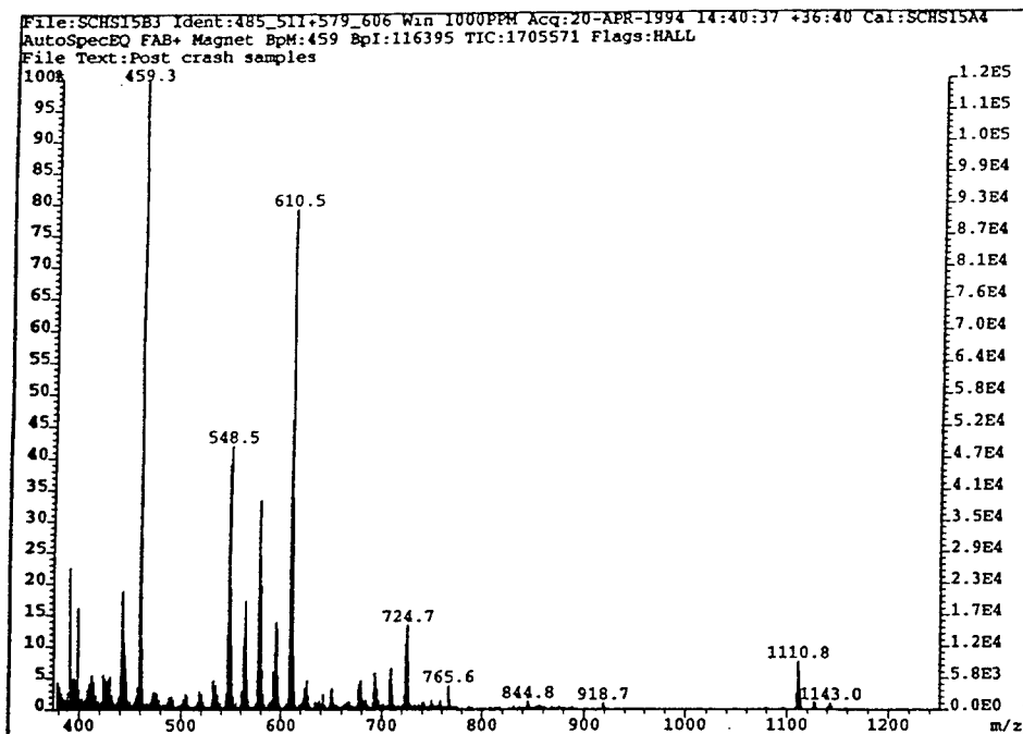
Figure 3.19: FAB + mass spectrum of of the polar band ( R_F=0.56 ) from alumina TLC of the reaction product of the MPPBDa derivatization.
