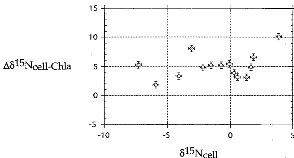
Figure 4.2: Plot of \Delta\delta^{15}\text{N}_{\text{cell-Chla}} vs \delta^{15}\text{N}_{\text{cell}} for the 14 algal cultures grown in this investigation. The y-error bar, 0.57 per mil, is the method precision for chlorophyll \delta^{15}\text{N} determinations in cultured phytoplankton. The x-error bar, 0.23 per mil, is the precision of \delta^{15}\text{N}_{\text{PON}} determinations in this study.
