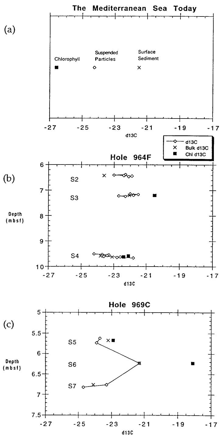
Figure 5.13: Carbon isotopes in (a) the modern Mediterranean Sea, and (b,c) Late Quaternary Eastern Mediterranean sediments. The particulate \delta^{13}\text{C} value is an average of 3 samples from the Eastern Mediterranean. The chlorophyll \delta^{13}\text{C} value is a single measurement from the western basin (see text).
