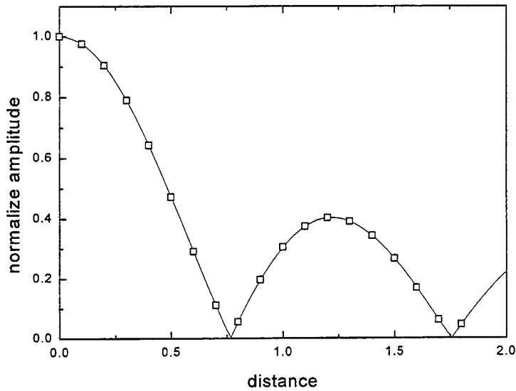
Fig 3.3 Suppression of a signal with frequency 50 by a pump of amplitude 10^{-2} and frequency 1. The signal's amplitude is normalized to its value of 10^{-4} at the origin. The points are the result of numerical integration, and the solid line corresponds to the theoretical expression (3.4). The amplitude of the signal was calculated by averaging over 10^6 cycles of the signal in the averaging.
