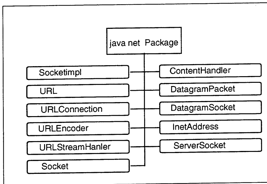
Figure 3.4 java.net Package
