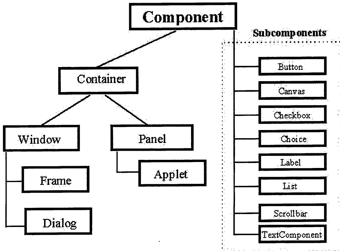
Figure 2 Structure of AWT
