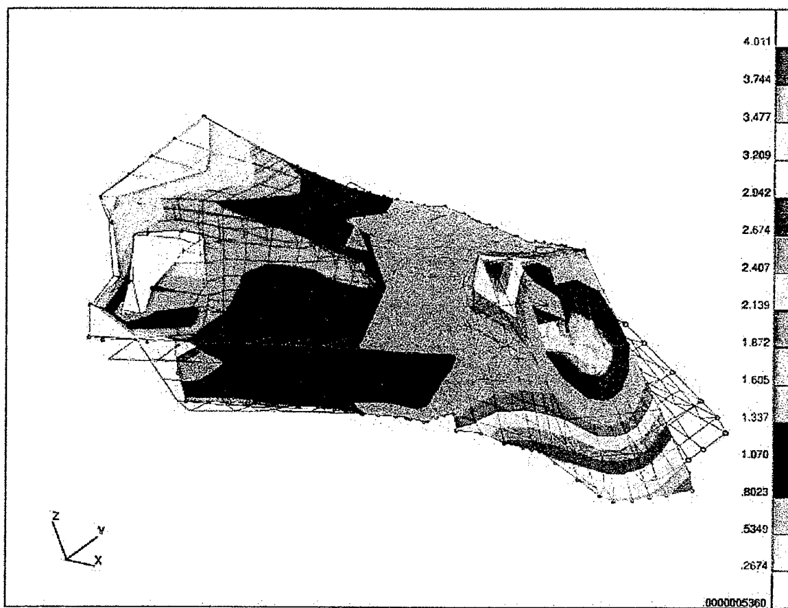
Figure 27: Torsion Displacement of Bulk-Mod Model
