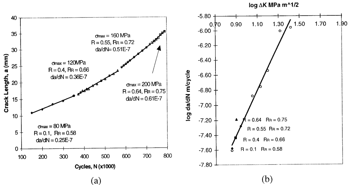
Figure 8. a) Plot of a Versus N for R Values as Shown for a Standard 7-Ply Test Specimen and b) Plot of \log da/dN Versus \log \Delta K_{\infty} for the Data From the 7-Ply Specimen ( R=0.1 ) of Figure 6b, Including, as Solid Data Points the Corresponding Results for Different R -Ratios From 8(a).
