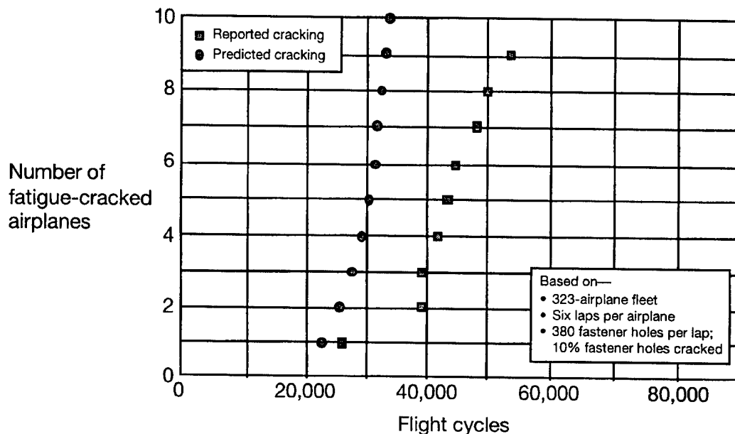
Figure 9. Comparison of Predicted and Actual Cracking Histories for Example 1 Problem.
