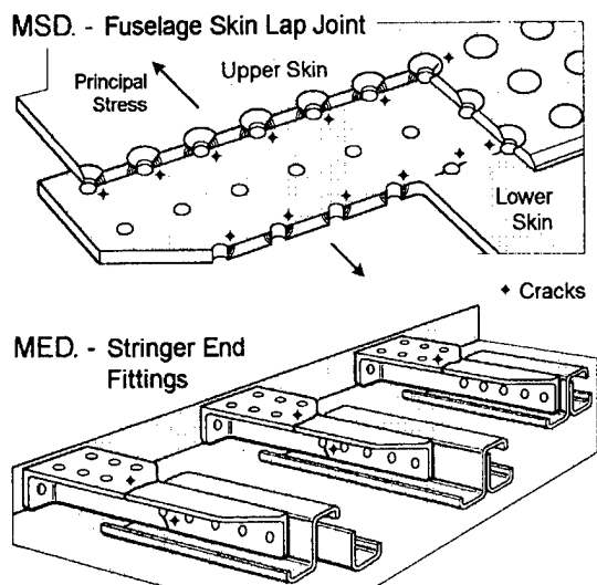
Figure 1. Examples of MSD and MED.
