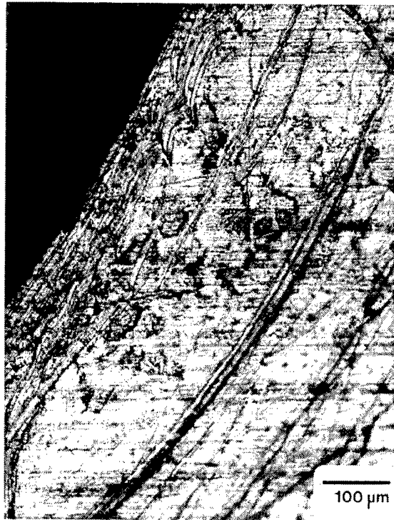
Figure 6. Photomicrograph of Microcracks Adjacent to Rivet Head Prior to the Emergence of a Propagating Radial Crack.
