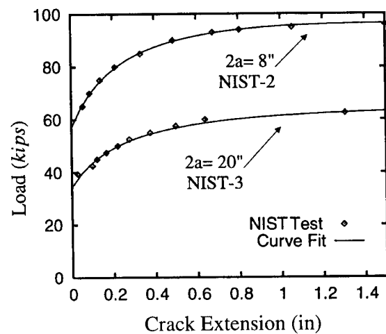
Figure 6. Experimental Data for NIST-90 MSD-2 and MSD-3.
