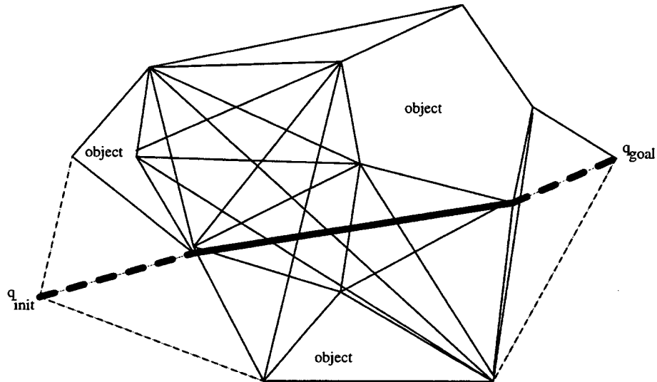
Figure 4. Visibility graph
