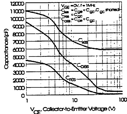
Fig. 8 - Typical Capacitance vs. Collector-to-Emitter Voltage
