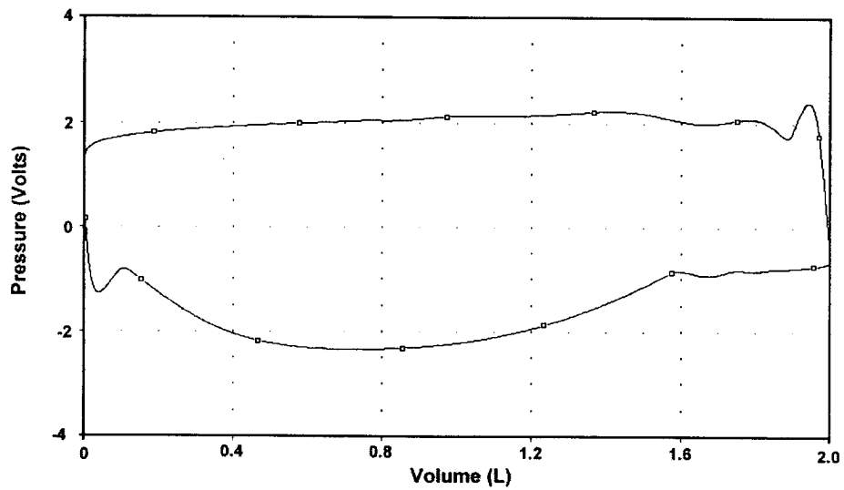
Figure 11. Simulated P-V loop for the above analog. Compare to Figure 6. (Model parameters: source voltage = 2.8v, constant current source=1A, R_{insp}=3 ohms, R_{exp}=0.2 ohms, L_{insp}=400 mH, L_{exp}=150 mH, C=4 mF, R_{shunt}=0.5 ohm.)
