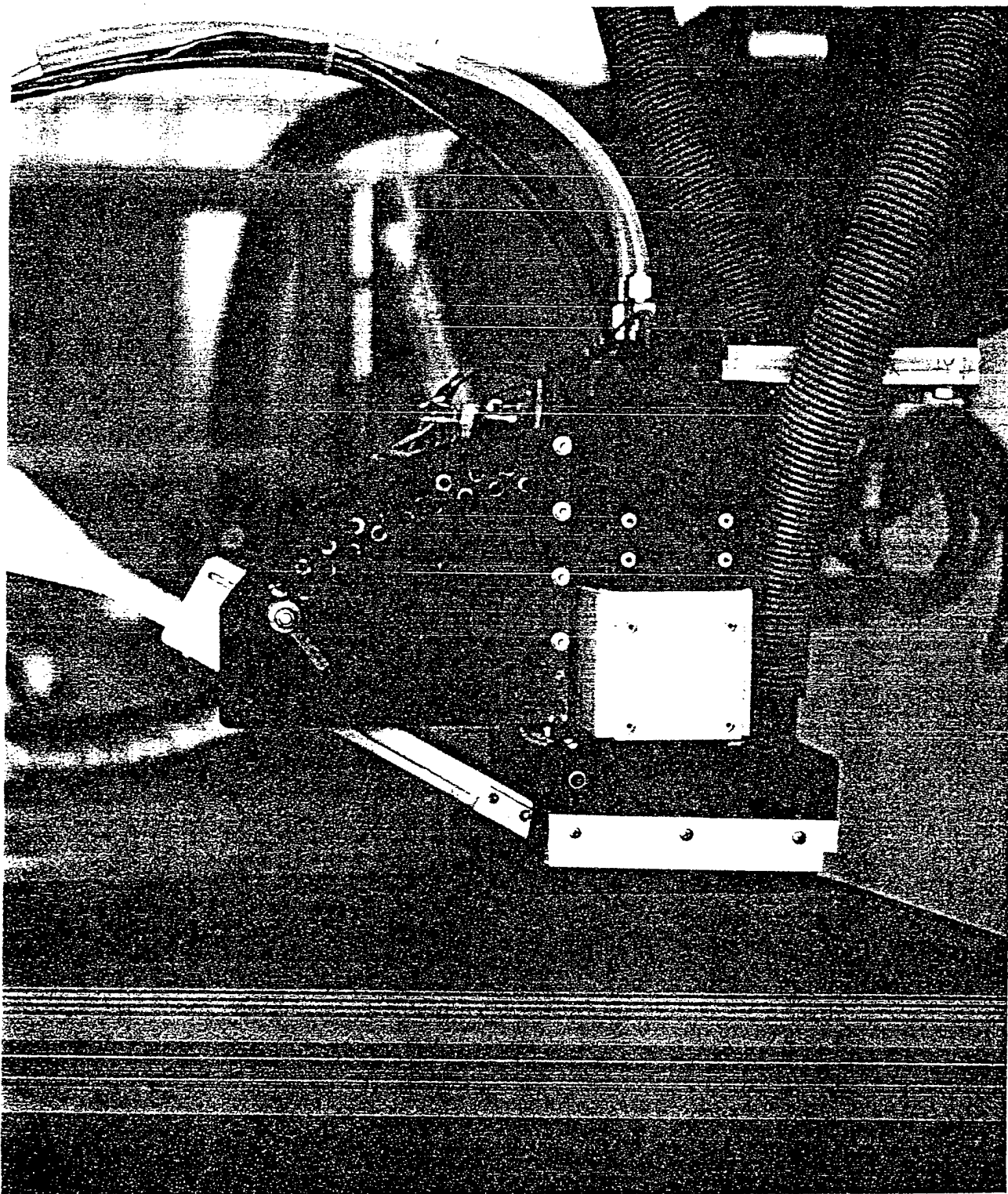
Figure 3. PRAM Stripping Head
