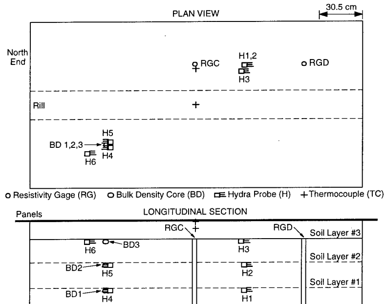
Figure 13. Instrument layout.
