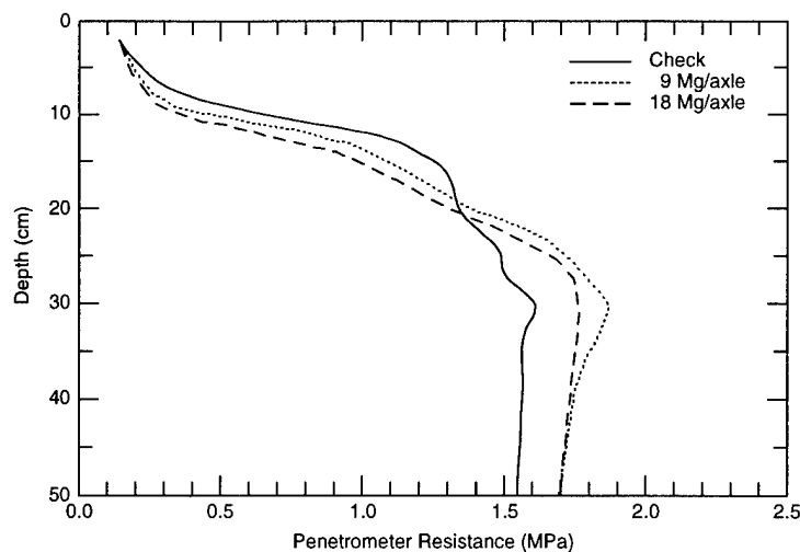
Figure 5. Penetrometer resistance 4 years after initial loading of Webster clay loam in Waseca, Minnesota, with a wheeled vehicle. (After Voorhees et al. 1986.)
