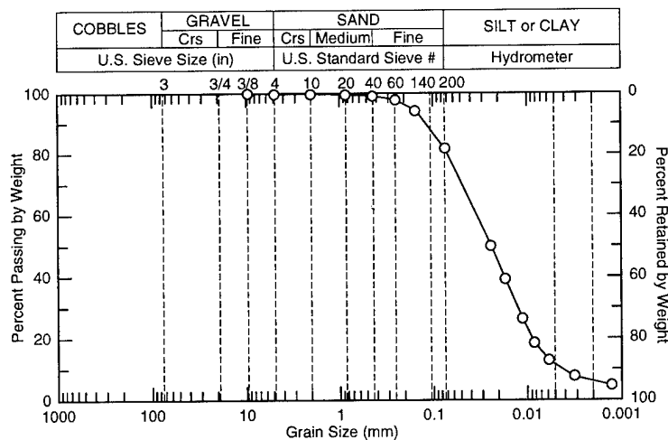
a. Grain size distribution (ASTM 1996a).
