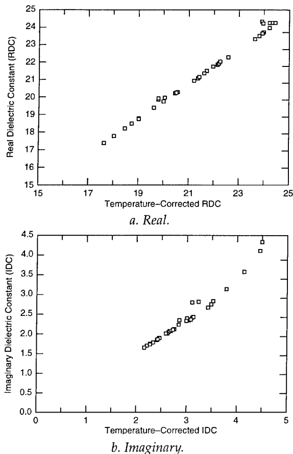
Figure 29. Dielectric constants vs. temperature-corrected constants.
