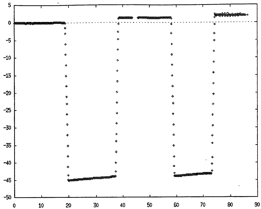
Figure 25: Roll Test: K_1 = 0.0 , \tau = 1000 , pScale = 4.01, 40^\circ/\text{sec}
