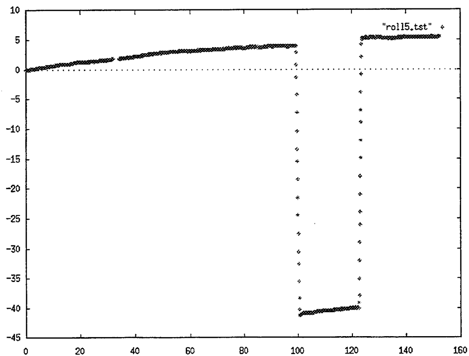
Figure 26: Roll Test: K_1 = 0.01 , \tau = 1000 , pScale = 4.01, 40^\circ/\text{sec}
