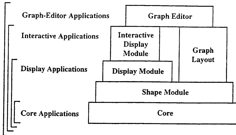
Figure 3.2: The Architecture of Grasper-CL. Grasper-CL's architecture is open and layered. Core applications use only Grasper-CL's core database function. Display applications utilize the shape and display modules, in addition to the core, to draw depictions of graph data structures. Interactive applications utilize the interactive display module and graph layout algorithms, in addition to the display, shape, and core components, to support direct user interaction with the graphical depictions of graph data structures. Graph-Editor applications utilize all of Grasper-CL's components to develop interactive graph editing systems with the look and feel of Grasper-CL's graph editor.
