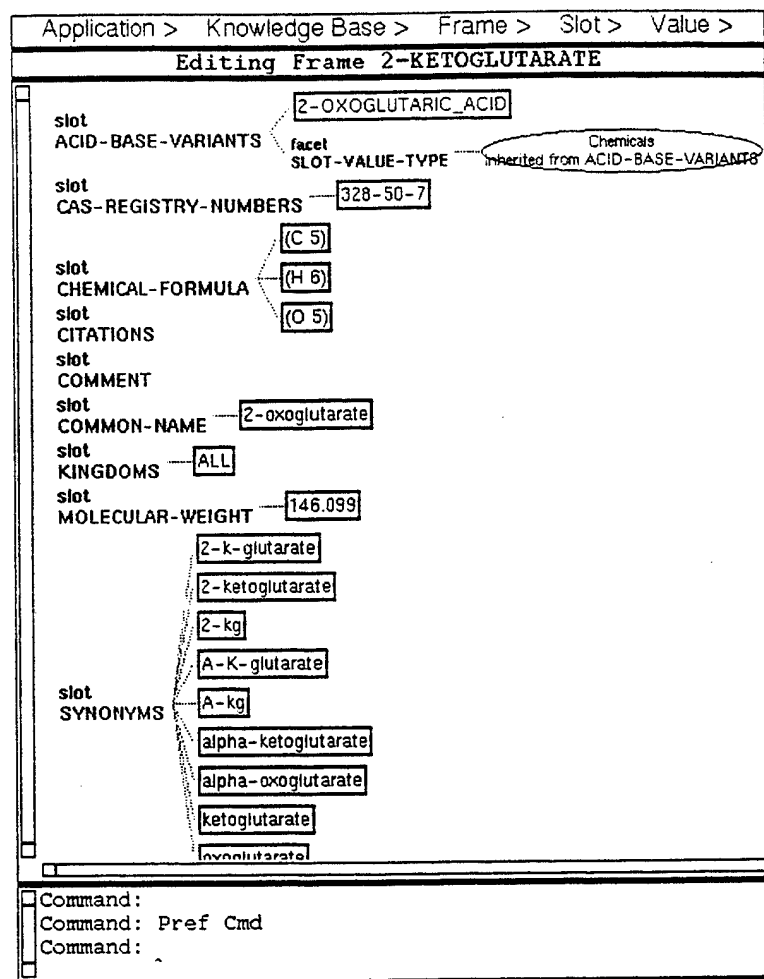
Figure 4.5: A sample frame-editing view for a chemical-compound frame. The slot-value-type facet on the acid-base-variants slot indicates that all values of this slot must be instances of the class Chemicals.
