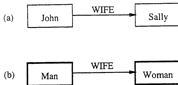
Figure 4.2: Examples of instance-level and class-level relationship graphs. (a) Instance-level relationship: the instance Sally is a value of the slot Wife in the instance John. (b) Class-level relationship: values of the slot Wife in instances of the class Man must be instances of the class Woman.
