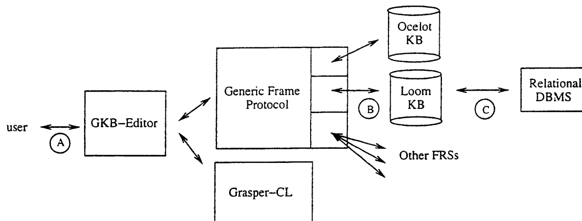
Figure 3.1: The architecture of the GKB-Editor system. All user interaction is through the GKB-Editor, which uses GFP to access KBs from a variety of FRSs, and Grasper-CL to generate and browse graphical displays.
