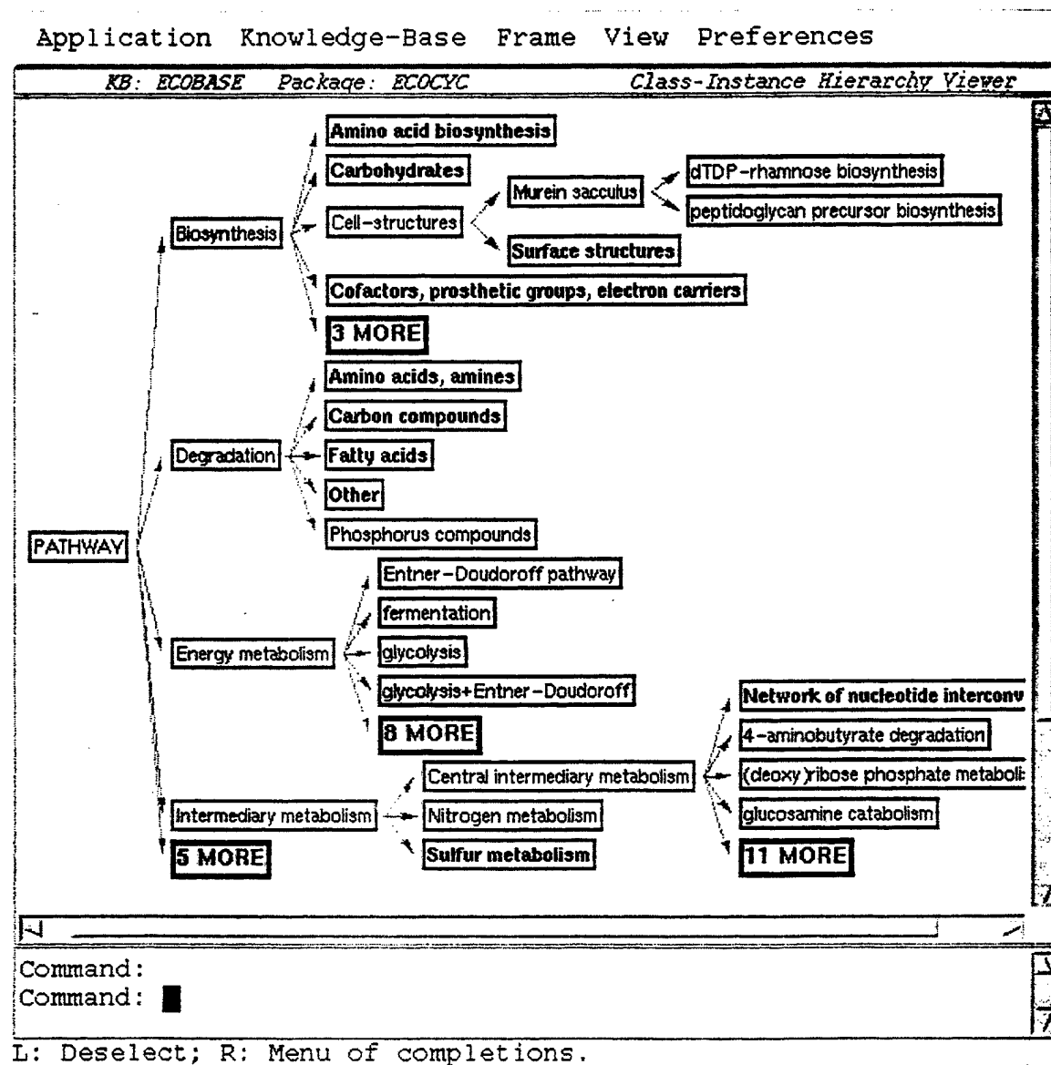
Figure S.1: A sample class/instance hierarchy view.
