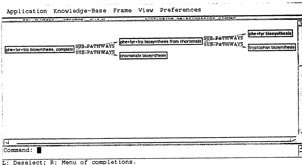
Figure 4.3: A sample instance-level relationships browse. Nodes with boldface labels can be further expanded. Double-headed arrows show bidirectional links, which are encoded by two slots that are mutual inverses.
