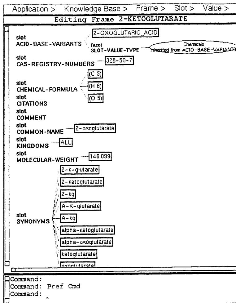
Figure S.3: A sample frame view.
