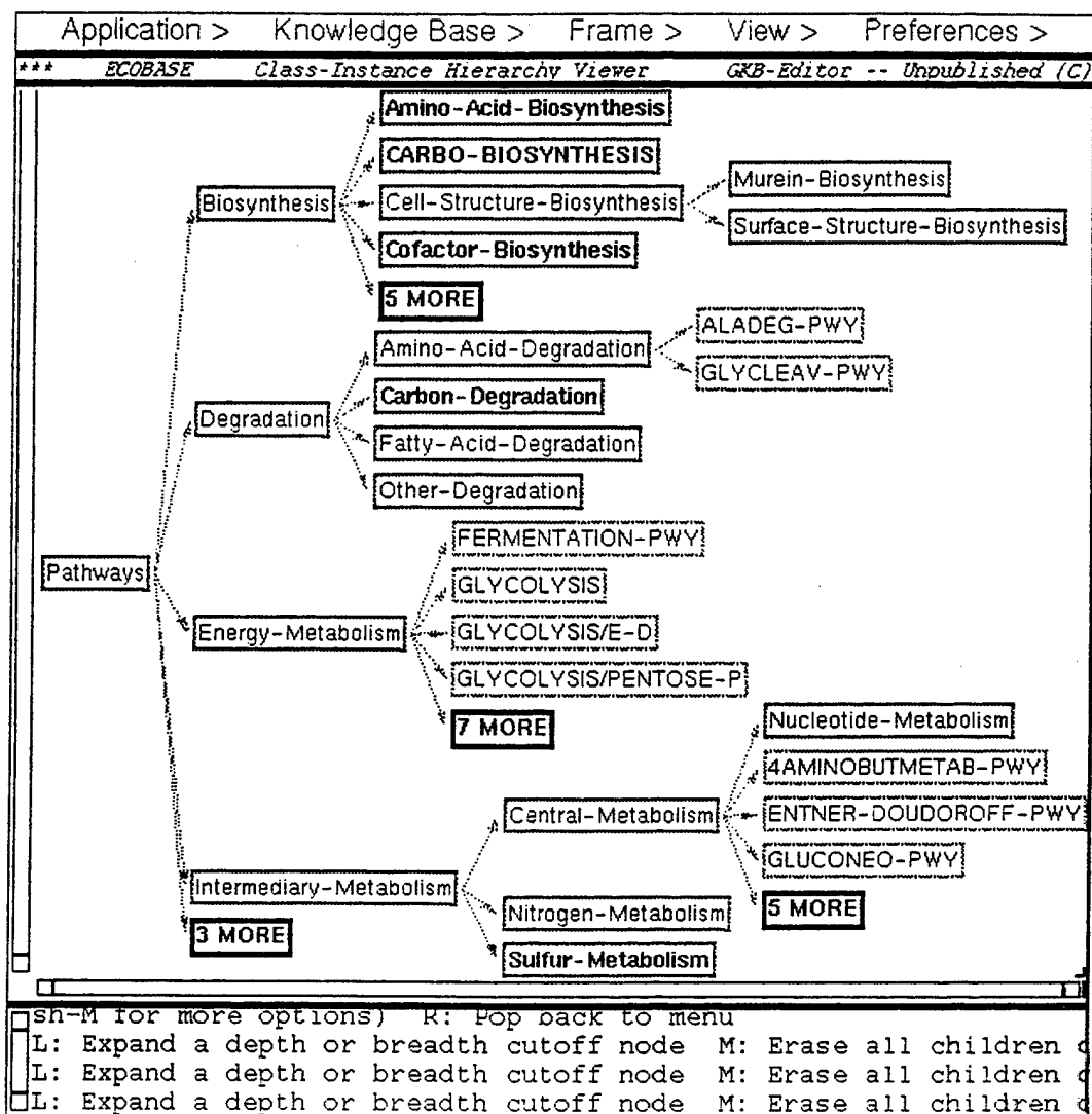
Figure 4.1: A sample class and instance hierarchy. Nodes whose labels are in boldface can be further expanded. Class frames have a solid border; instance frames have a gray border. Class names shown in bold can be expanded to show additional subclasses or instances. The "N More" nodes are "breadth cutoff nodes" that can also be expanded to show additional classes or instances.
