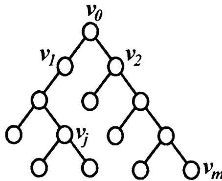
Figure 2. An enumeration tree.
