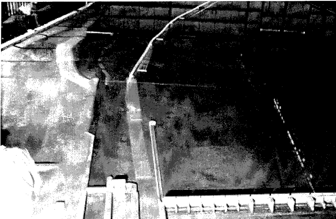
Photo 28. Lock Location 4, Plan A, looking upstream, discharge 65,000 cfs, path of down-bound tow approaching 1,200-ft lock
