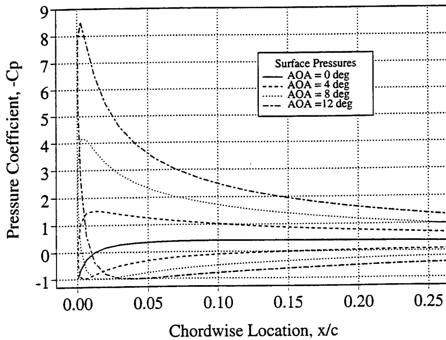
Figure 6.1. Surface Pressure Distribution Near the Airfoil Leading Edge, UPOT. \alpha = 0^\circ, 4^\circ, 8^\circ and 12^\circ .
