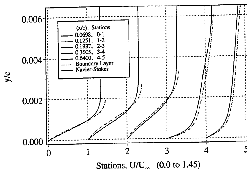
Figure 6.22. Boundary-Layer Velocity Profile Comparisons (N-S and Panel/Boundary-Layer Codes), \alpha = 4^\circ , Re = 540,000 ; N - S Analysis, M_\infty = 0.3 .
