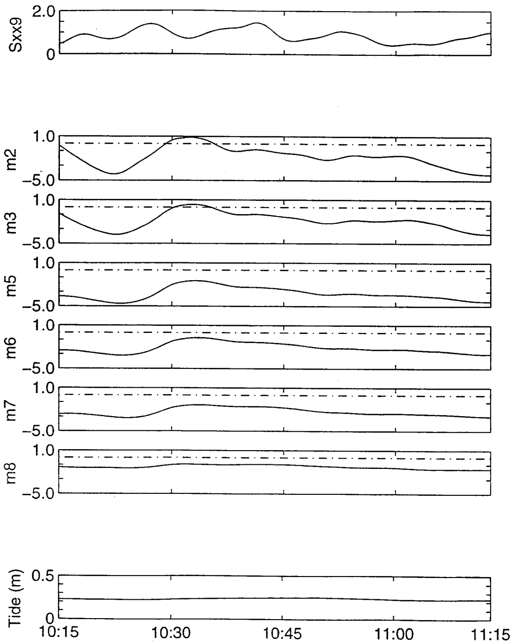
Figure 5. Top panel represents the offshore forcing, S_{xx} ( \text{J/m}^2 ), measured at p7. The next six panels m2-m8 depict the mean surface elevation (m) time series acquired by the manometer tubes. These values are a measure of the difference between the mean surface elevation at that location and the mean surface elevation furthest offshore. The bottom panel is the tidal elevation time series.
