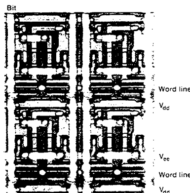
Figure 14. Schematic and microphotograph of BiFET memory cell.
