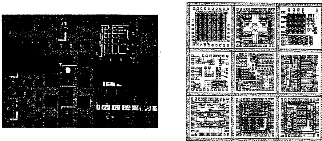
Figure 2: LEFT: A completed EoE optoelectronic integrated circuit with one of the integrated light emitting diodes in operation. The central emitting area of the LED is 11.5 \mu\text{m} by 16 \mu\text{m} , and the DGW in which it was grown is 50 \mu\text{m} square. RIGHT: The layout of the OPTOCHIP, a 7 mm square EoE OEIC chip combining designs from 9 research groups from the US and Canada, currently being processed at MIT.
