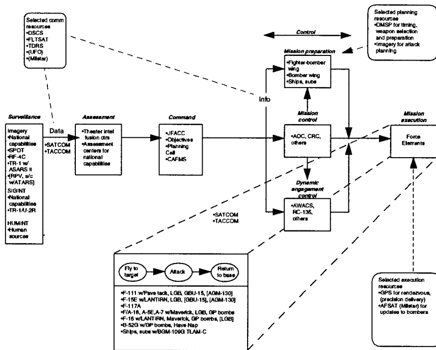
Figure 9. JFACC Operational (Static) Architecture 5
