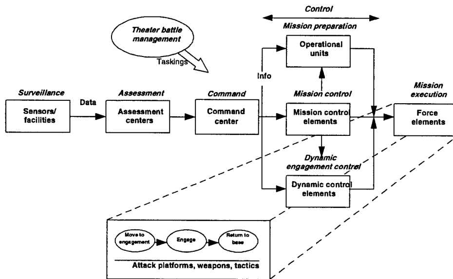
Figure 8. JFACC Functional Decomposition 3
