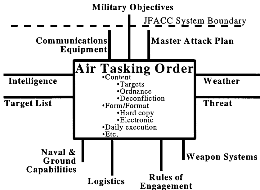
Figure 10. Air Tasking Order Data (Informational) Model
