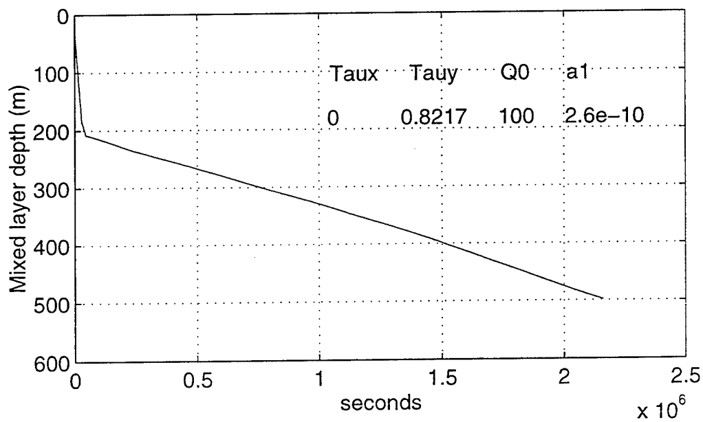
Figure 7. With 100 \text{ W/m}^2 of cooling, the model deepens the mixed layer 50% more when thermobaricity is included in the calculation ( a_1 \neq 0 ). Wind stresses Taux and Tauy are in dynes/cm 2 ; heating Q0 is in W/m 2 ; and a_1 is in (cm °C) -1 .
