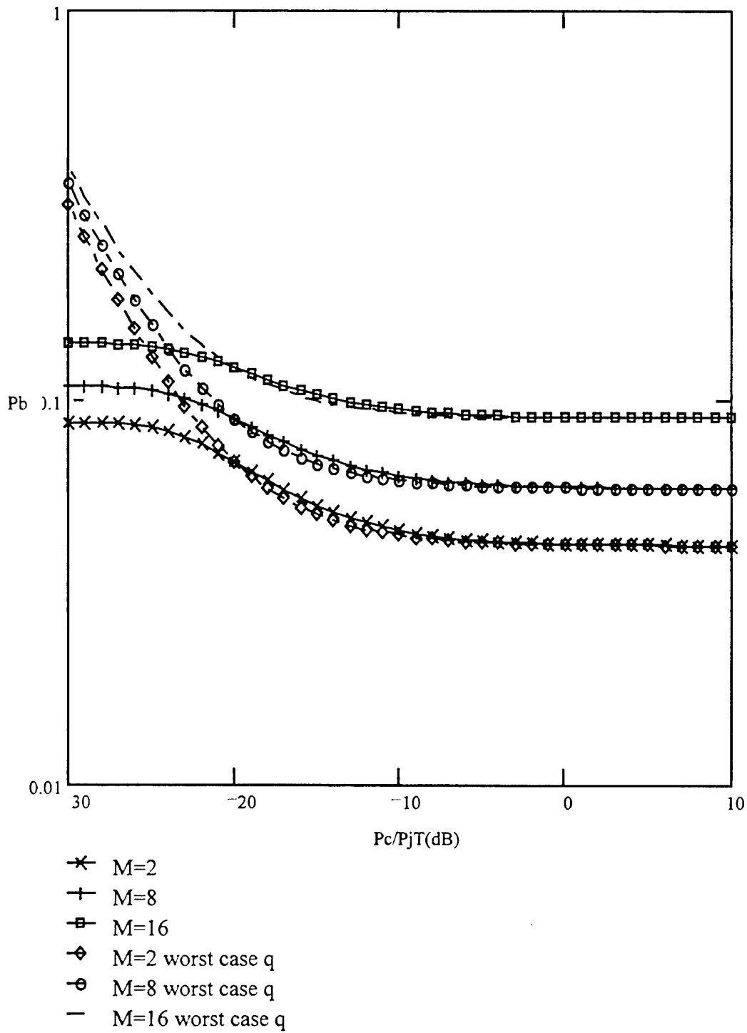
Figure 15 : Checking the Union Bound accuracy for Rayleigh fading of the information signal for band multitone interference with essentially no fading of the jammer tones, for both q = 100 and q_{wc} , for M = 2, 8, \text{ and } 16 . Anomaly detected!!! For increasing M the probability of error increases.
