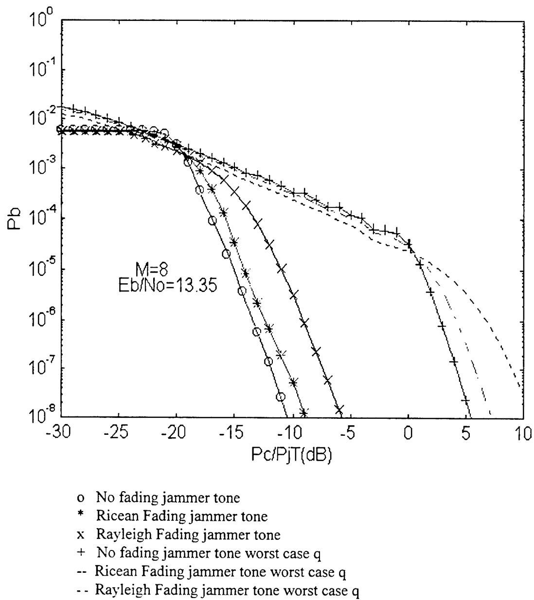
Figure 19: Performance of a FH/8FSK non-coherent receiver with essentially no signal fading and various interference fading for independent multitone interference.
