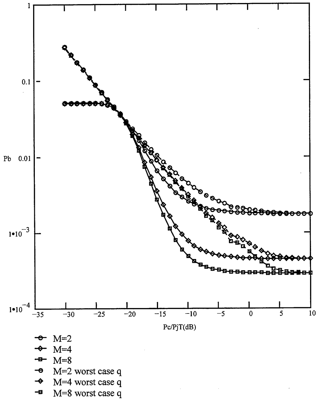
Figure 12: Checking the Union Bound accuracy for Ricean fading of the information signal for band multitone interference with essentially no fading of the jammer tones, for both q = 100 and q_{wc} , for M = 2, 4 , and 8 . No anomaly detected for the P_b using the union bound and P_b decreases as M increases.
