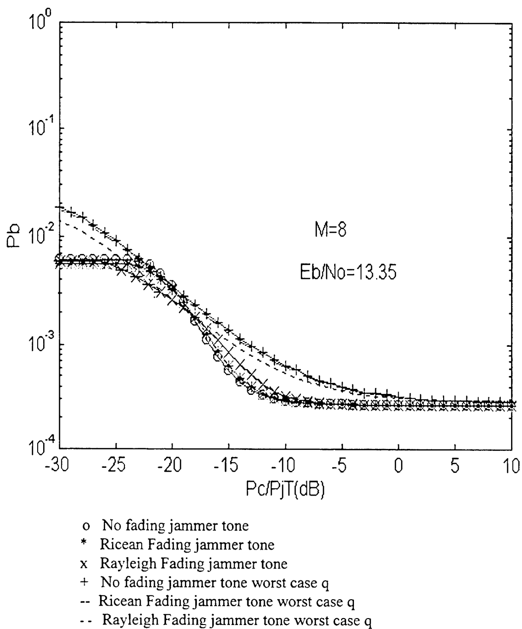
Figure 21: Performance of a FH/8FSK non-coherent receiver with Ricean signal fading and various interference fading for independent multitone interference.
