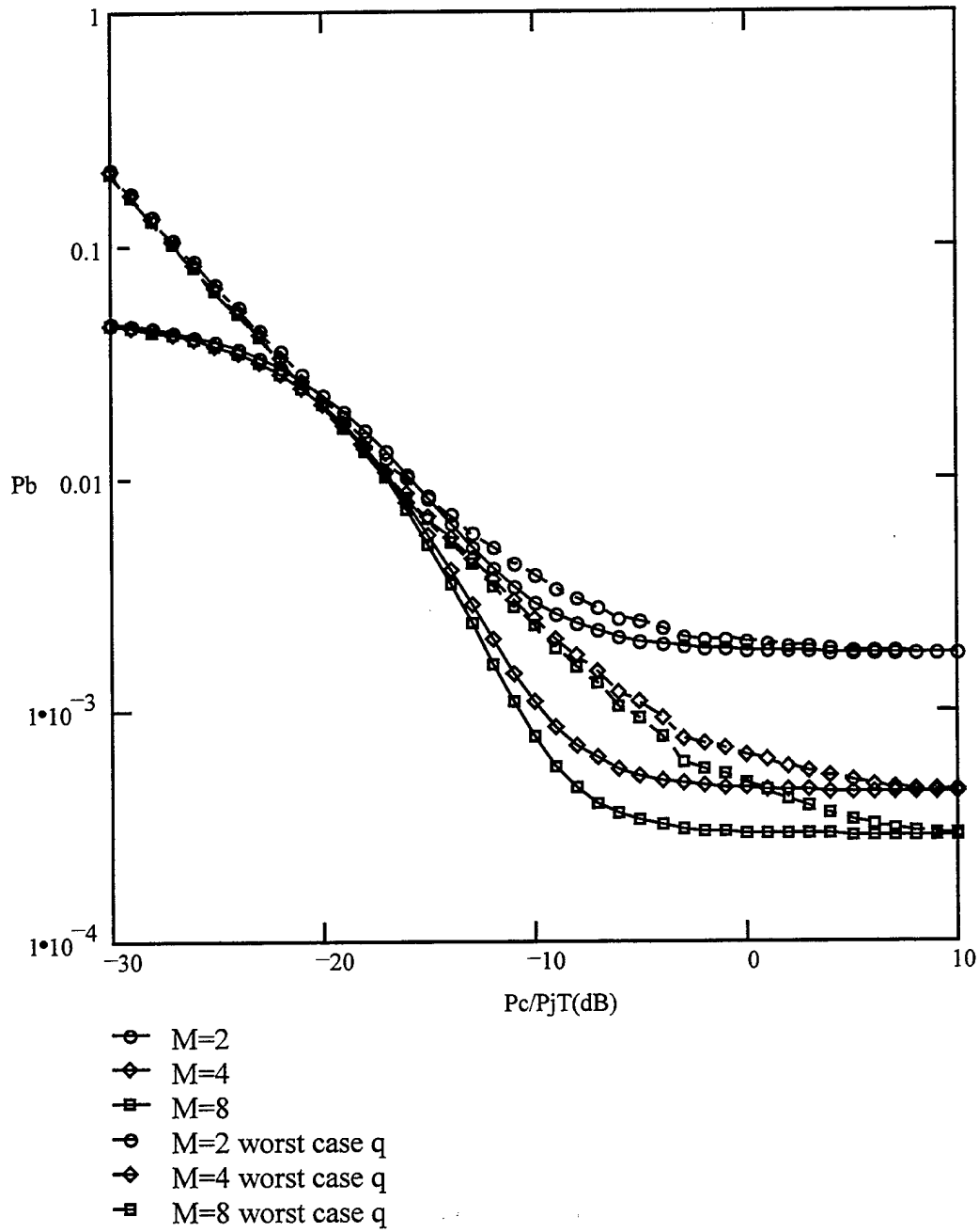
Figure 14: Checking the Union Bound accuracy for Ricean fading of the information signal for band multitone interference with Rayleigh fading of the jammer tones, for both q = 100 and q_{wc} , for M = 2, 4 , and 8 . No anomaly detected for the P_b using the union bound and P_b decreases as M increases.
