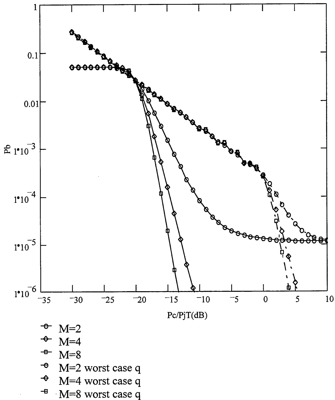
Figure 10: Checking the Union Bound accuracy for essentially no fading of the information signal for band multitone interference with no fading of the jammer tones, for both q = 100 and q_{wc} , for M = 2, 4, \text{ and } 8 . No anomaly detected for the P_b using the union bound and P_b decreases as M increases.
