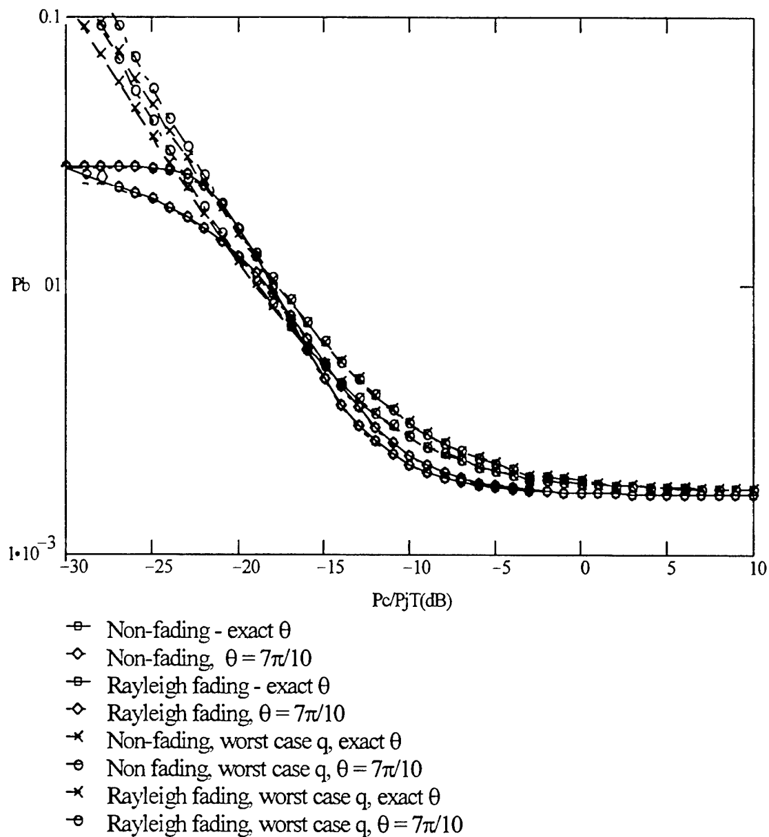
Figure 25: A comparison of the union bound curves for a FH/BFSK noncoherent receiver's performance with Ricean information signal fading for independent multitone interference with either no fading or Rayleigh fading of the jammer tones, with q = 100 and worst case q , obtained by integrating \theta and also by approximating \theta with \frac{7}{10}\pi . The results obtained are identical, so the approximation can effectively be used simplifying the calculations.
