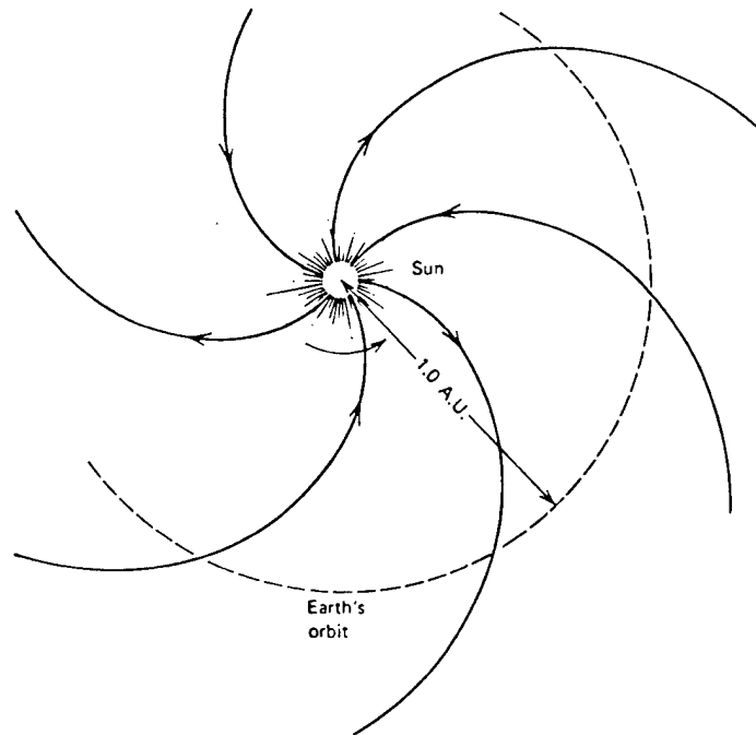
Figure 21B. Schematic representation of the Archimedes spiral structure of the interplanetary magnetic field in the ecliptic plane, (Haymes 6 , p.284).
