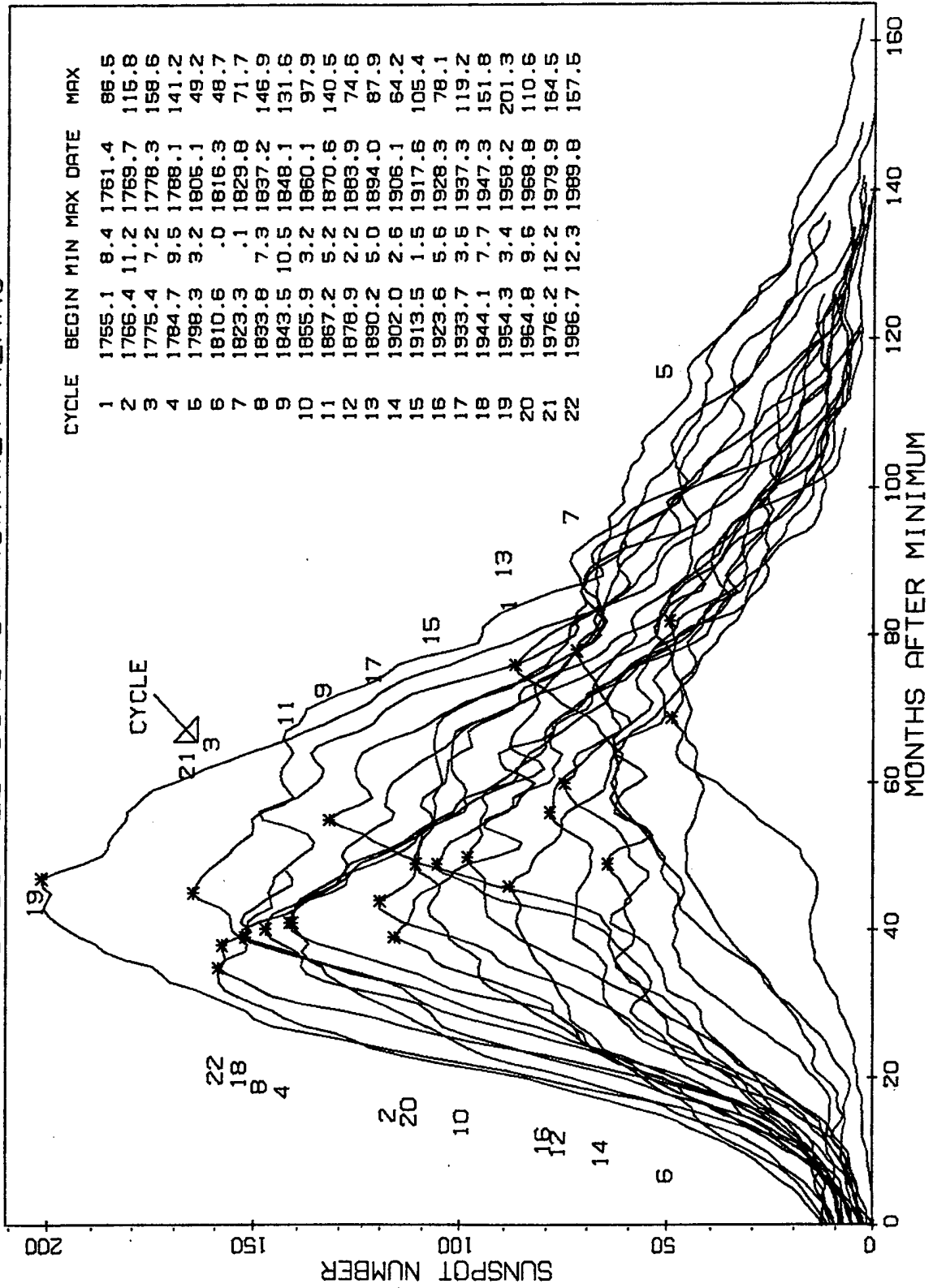
Figure 14. Monthly mean smoothed sunspot number for individual solar cycles.
