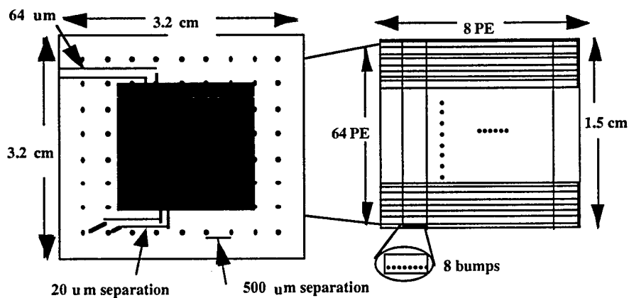
Figure 21: back side of compander and processing chip (left) and front side of processing chip (right).
